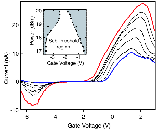
FIG. 4 (color online). SAW-induced current versus gate voltage for fixed values of rf power 17.3 (blue), 17.9, 18.8, 19.1, 19.4, 19.7, and 20 dBm (red). Inset: Points correspond to |I_{\text{SAW}}| = 0.1 nA. This small threshold current was arbitrarily chosen to indicate the region in the P - V_g plane in which a SAW-induced current is absent. The dashed lines are a guide to the eye.
