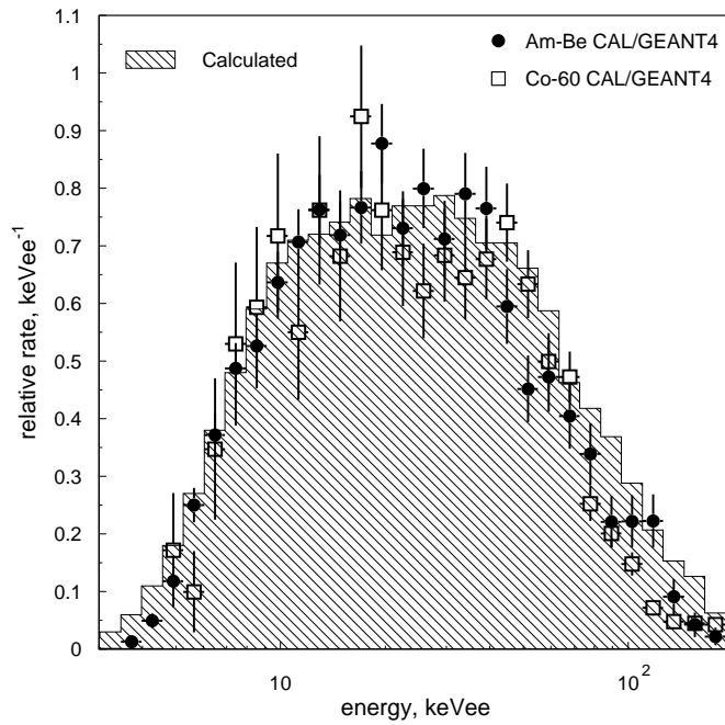
Fig. 11. Comparison of the overall nuclear-recoil detection efficiency, calculated as described in § 3.4, with the relative efficiencies obtained by dividing the actual AmBe and 60 Co calibration spectra by the simulated energy dependencies obtained for single scatters in a detector with unity efficiency. Although the calibration data have been scaled to match the calculated efficiency (hatched region), the good agreement in spectral shape supports the calculations summarised in Table 2.
