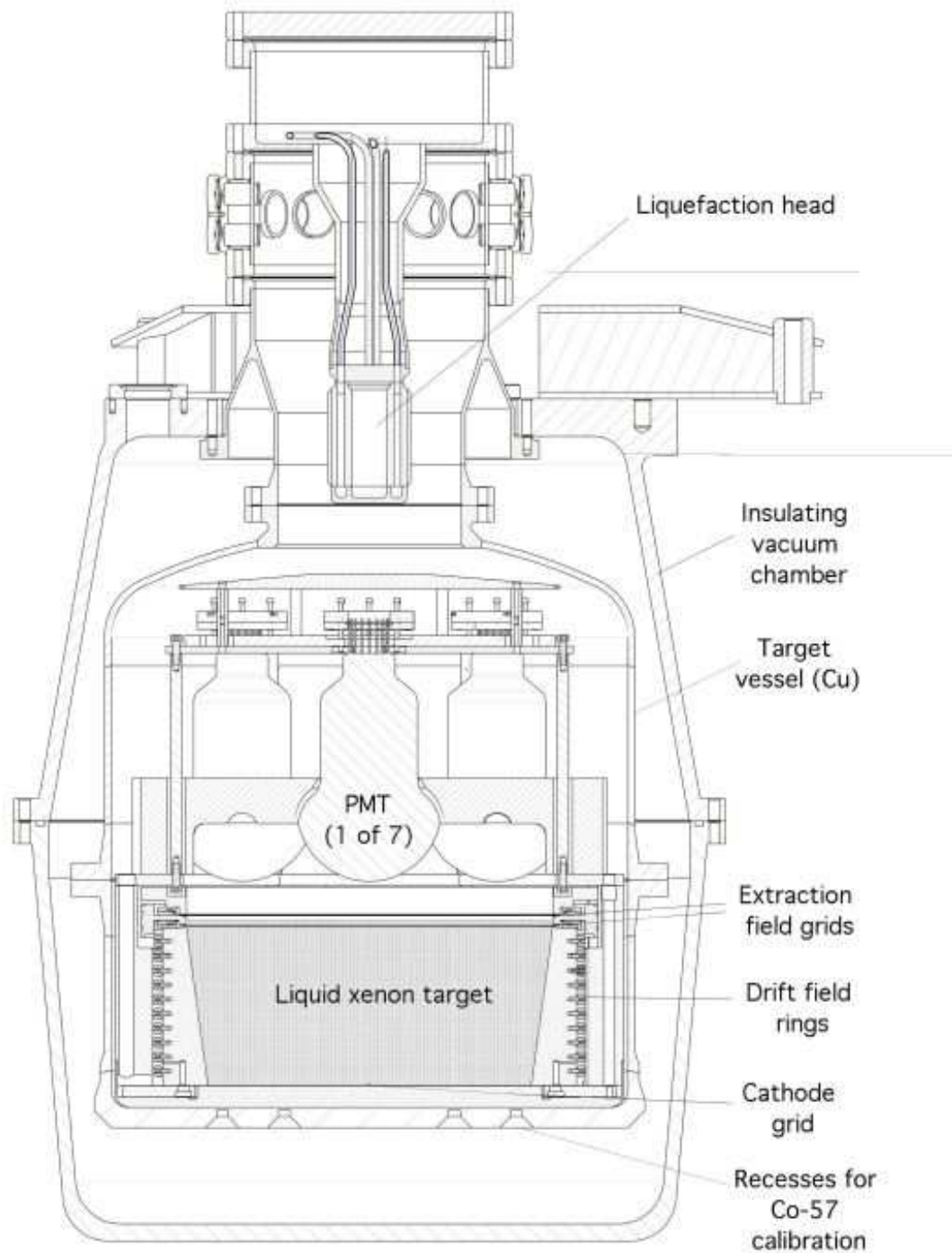
Fig. 1. Schematic of the ZEPLIN-II detector. The liquid xenon volume is shown, viewed from above by 7 quartz-window photomultipliers. The electrode arrangement defines a drift region between the cathode grid and the lower extraction grid where the field is parallel and uniform (this is obtained with the help of lateral field-shaping rings embedded in the PTFE walls). The extraction region (where electroluminescence is generated) is defined by the two grids located either side of the liquid surface. Xenon liquefaction occurs on the liquefaction head, with liquid dripping onto a copper shield which deflects it away from the photomultiplier array and the active volume.
