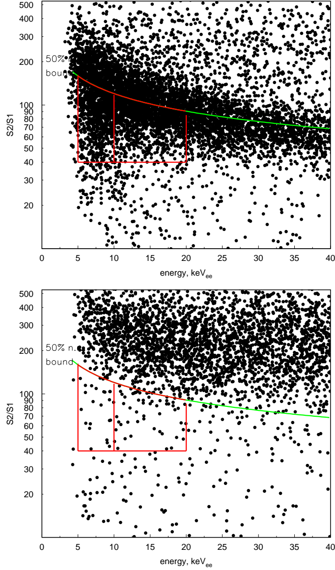
Fig. 8. Calibration using neutrons from an AmBe source (upper) and Compton scattered 60 Co γ-rays (lower). These calibrations were performed at a high trigger rate, leading to a small, uniform, population of coincidental events distributed throughout the S2/S1 parameter space. These coincidentals are verified by comparison with events with unphysical drift times. Also shown are the S2/S1 boundary for 50% nuclear recoil acceptance, and the acceptance window used in the dark matter analysis.
