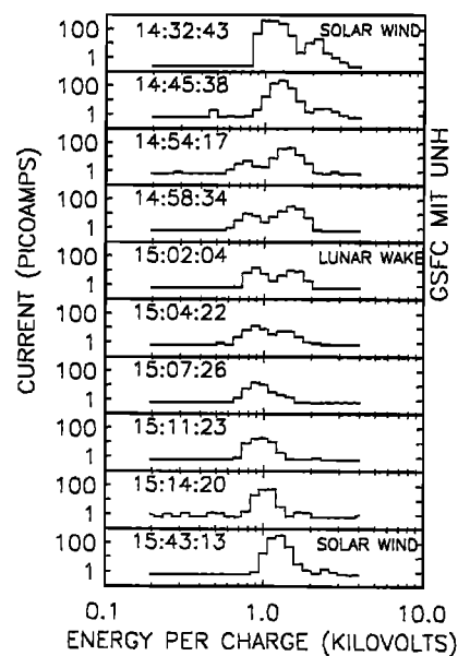
Figure 2. Time sequence of Faraday cup current versus energy/charge spectra as WIND crossed the wake. At 14:32 UT, signal peaks are due to solar wind \text{H}^+ and \text{H}_\alpha^{++} , with (density \text{H}_\alpha^{++} )/(density \text{H}^+ ) = 0.025. At 15:02 UT there are two \text{H}^+ signal peaks. At 15:43 UT, peak signals due to solar wind \text{H}^+ and a small flux of \text{H}_\alpha^{++} .
