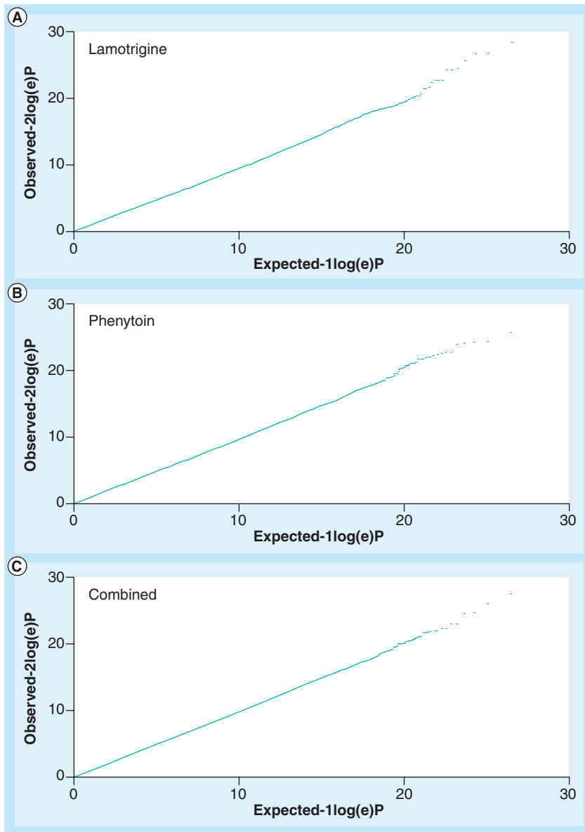
Figure 2. Quantile–quantile plot of the association results. Quantile–quantile plots of p-values from genome-wide association studies of (A) lamotrigine, (B) phenytoin and (C) total drug-induced cutaneous adverse drug reactions vs controls calculated using logistic regression and including significant EIGENSTRAT axes as covariates. The expected chi distribution is represented along the x-axis, while the observed chi distribution is represented along the y-axis. Figure generated in WGAViewer.
