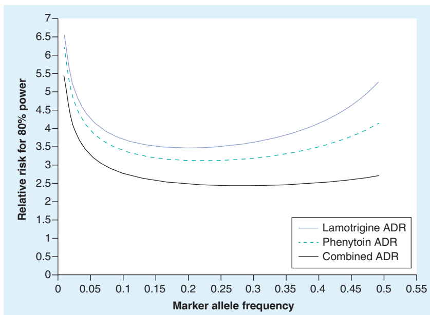
Figure 3. Power calculation for genome-wide association results.
