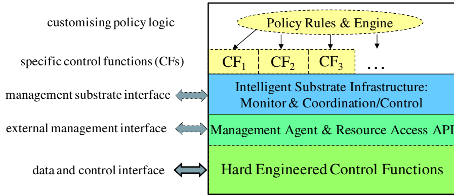
Figure 2. Self-managed node architecture
