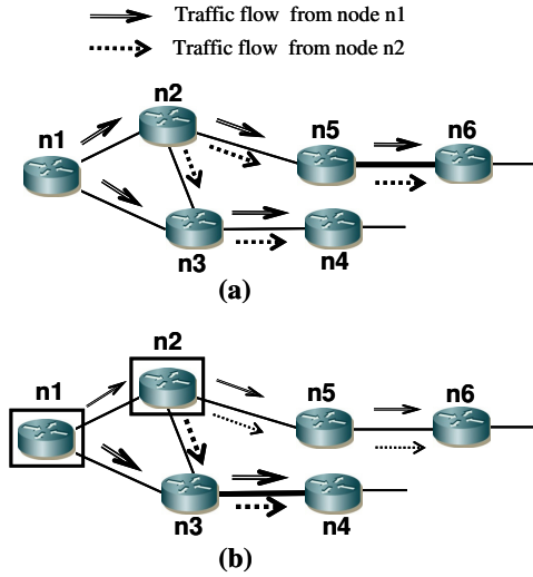
Figure 3. Example of conflicting decisions between ingress nodes n1 and n2
