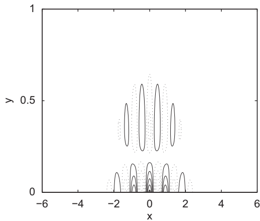
Fig. 7. The real part p(x,y,-h) of the bottom pressure for the fundamental l CTW mode \omega_{0,1} as a function of x and y at z = -h(x,y) , for the depth profile 1(c,d) with B=0.25 and b(z) held constant.
