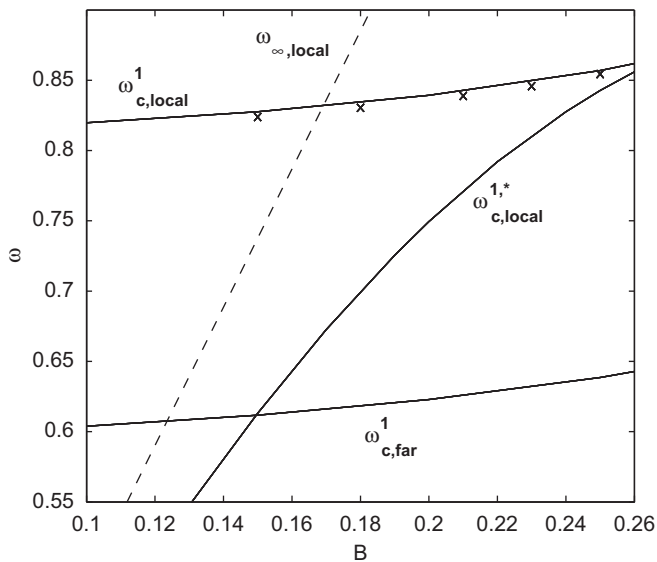
Fig. 6. The fundamental l CTW frequency, denoted by the crosses, as a function of B for the topography shown in Fig. 1(c,d).
