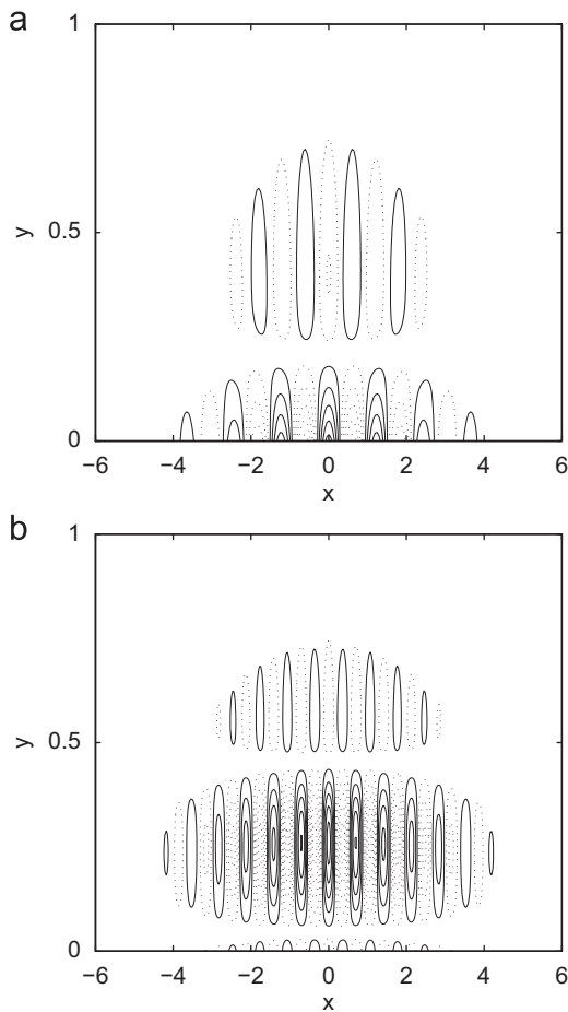
Fig. 4. The real part of the bottom pressure p(x,y,-h) for (a) the fundamental l CTW mode \omega_{0,1} and (b) the l CTW mode \omega_{0,2} for the depth profile 1(a,b) with B=0.01 and b(z)\equiv 1 . The contours are at equal intervals with negative values dashed and the zero contour omitted.
