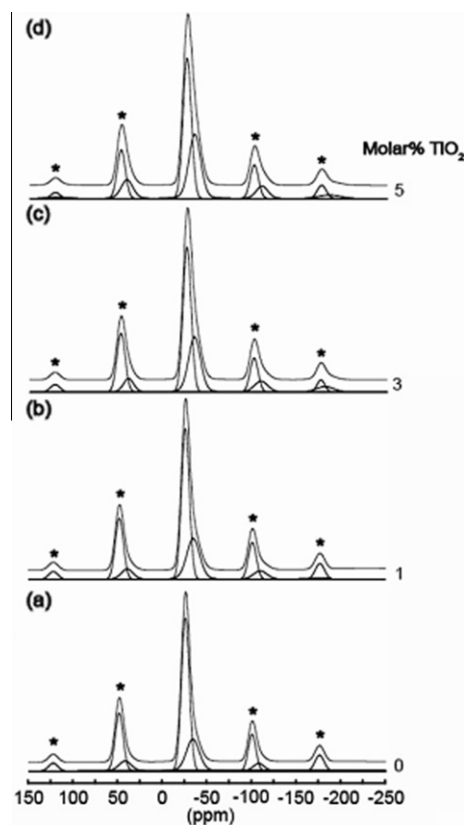
Fig. 8. 31 P MAS-NMR spectra obtained for the glass samples with increasing mol.% TiO 2 : (a) Ti-free, (b) TiO 2 1 mol.%, (c) TiO 2 3 mol.% and (d) TiO 2 5 mol.%. The asterisks represent the deconvoluted spinning sidebands.
