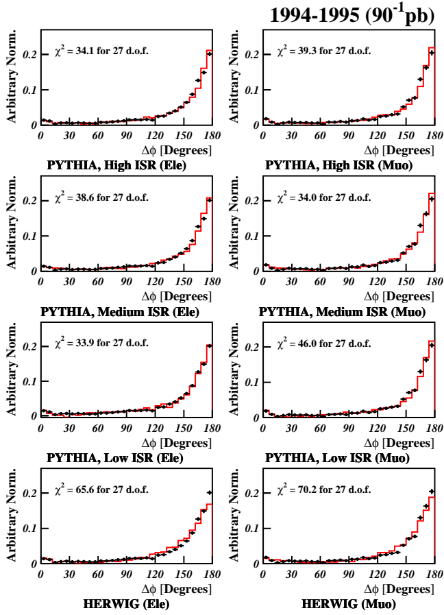
FIG. 7: Comparisons between the shape of the tag \Delta\phi distribution for data (points) and the tag \Delta\phi distribution predicted by the various Monte Carlo samples (line). In these comparisons, the normalizations of each production mechanism were allowed to vary independently and were chosen to give the best fit between the Monte Carlo and the data. Again, the fit \chi^2 takes into account Monte Carlo statistics in addition to errors on the data.
