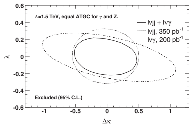
FIG. 3. Limits at 95% C.L. on ATGC using WW and WZ decays to \ell\nu jj , W\gamma decays to \ell\nu\gamma , and the combination of both channels.
