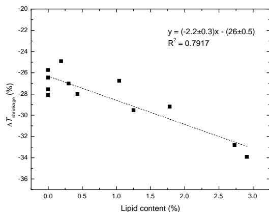
Figure 1. Decrease in shrinkage temperature of parchment samples from 1965 and 2005 during accelerated ageing, in dependence of their lipid contents.
