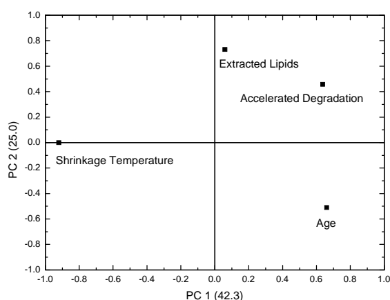
Figure 2. Principal component analysis loading plot for the principal component analysis of data for Set I: shrinkage temperature of all samples, age of samples, extracted lipids (%), and accelerated degradation (whether carried out or not).
