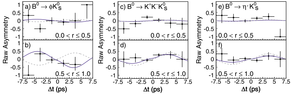
FIG. 2 (color online). (a) The asymmetry, A , in each \Delta t bin for B^0 \rightarrow \phi K_S^0 with 0 < r \leq 0.5 , (b) with 0.5 < r \leq 1.0 , (c) for B^0 \rightarrow K^+ K^- K_S^0 with 0 < r \leq 0.5 , (d) with 0.5 < r \leq 1.0 , (e) for B^0 \rightarrow \eta' K_S^0 with 0 < r \leq 0.5 , and (f) with 0.5 < r \leq 1.0 , respectively. The solid curves show the result of the unbinned maximum-likelihood fit. The dashed curves show the SM expectation with \sin 2\phi_1 = +0.731 and \mathcal{A} = 0 .
