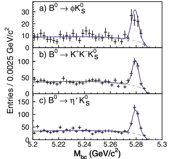
FIG. 1 (color online). The M_{bc} distributions for (a) B^0 \rightarrow \phi K_S^0 , (b) B^0 \rightarrow K^+ K^- K_S^0 , and (c) B^0 \rightarrow \eta' K_S^0 within the \Delta E signal region. Solid curves show the fit to signal plus background distributions, and dashed curves show the background contributions. The fit functions are the same as those used in the previous publication [9].
