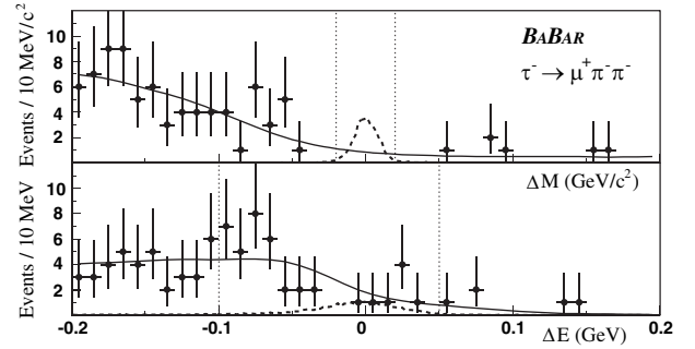
FIG. 2. Data (points) and background expectation (solid line) are shown for the \mu^+\pi^-\pi^- candidates displayed in Fig. 1. Expected signal distributions for a branching fraction of 5 \times 10^{-7} are also shown as the dashed curve. The vertical lines indicate the signal region.
