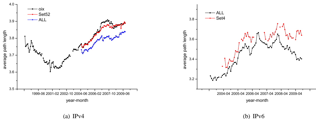
Figure 5: Evolution of the average shortest path length of the IPv4 and IPv6 networks.
