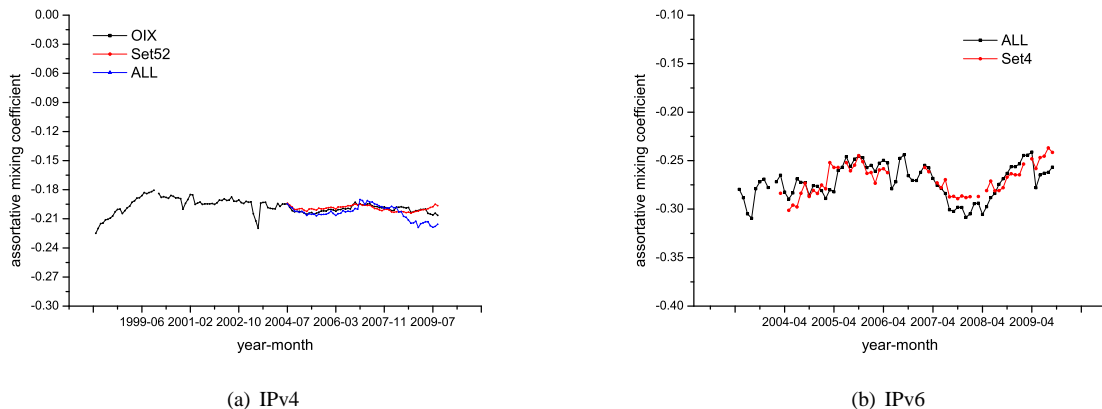
Figure 8: Evolution of the assortative coefficient of the IPv4 and IPv6 networks.
