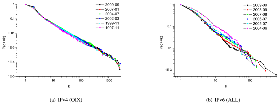
Figure 6: Evolution of degree distributions in the IPv4 and IPv6 networks.
