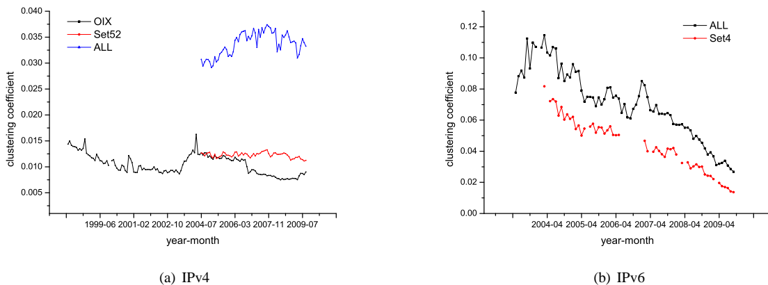
Figure 7: Evolution of clustering coefficients in the IPv4 and IPv6 networks.
