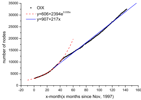
(c) Curve fittings for IPv4 (OIX)
