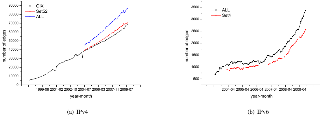
Figure 2: Evolution of the number of edges of the IPv4 and IPv6 networks.
