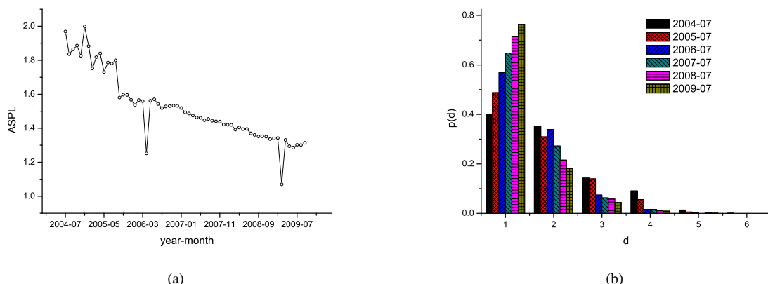
Figure 9: The impact of IPv6-over-IPv4 tunnelling on the Internet evolution. (a) Evolution of the average shortest path length (ASPL) of the connected IPv6 AS pairs on the IPv4 network. (b) Evolution of the distribution of shortest path length of the connected IPv6 AS pairs on the IPv4 network, where p(d) is the probability that a connected pair of ASes on the IPv6 network has path length d on the corresponding IPv4 network.
