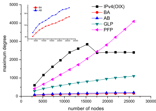
Figure 10: Evolution of maximum degree of real AS topology(OIX) and four typical generative models. BA network is generated with m=2 [14]. AB network is generated with p=0.2 , q=0.3 and m=2 [15]. GLP network is generated with p=0.4695 and \beta=0.6447 [16]. PFP network is generated with p=0.4 and \delta=0.021 [18]. Evolution of maximum degrees in BA and AB is further illustrated in the inset since the growth trends are not legible in the original plot due to the relatively small absolute values.
