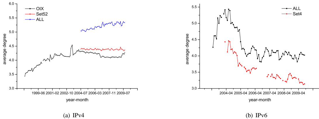
Figure 4: Evolution of the average degree of the IPv4 and IPv6 networks.
