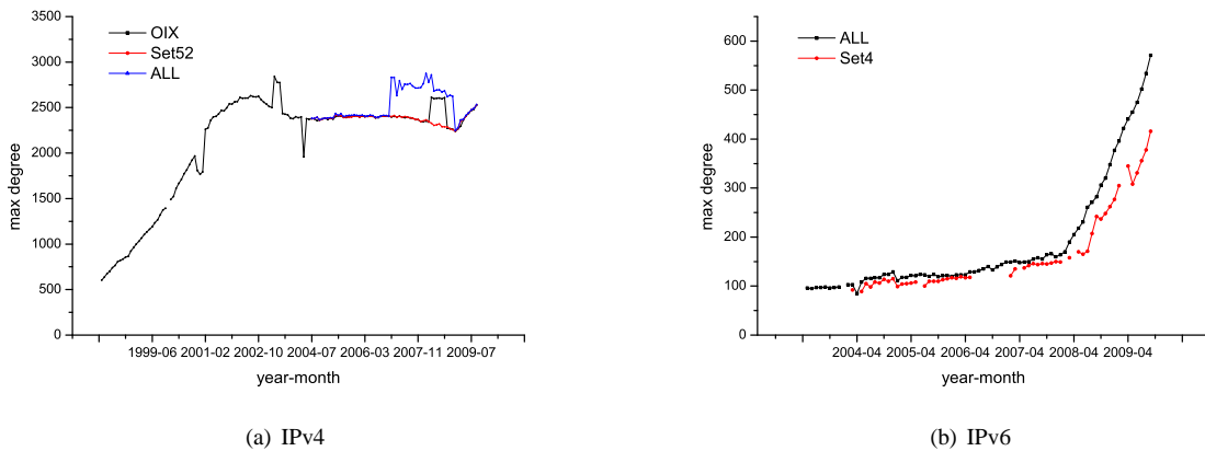
Figure 3: Evolution of the maximum degree of the IPv4 and IPv6 networks.
