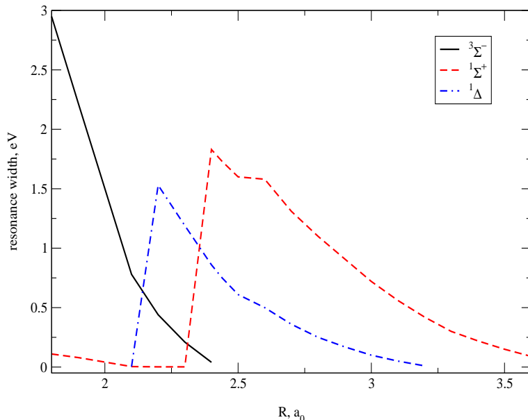
Figure 6. Resonance width as a function of C-F bond length. Solid line represents a width of the shape resonance of {}^3\Sigma^- symmetry. Dashed and dot-dashed lines represent a width of the shape resonances of {}^1\Sigma^+ and {}^1\Delta symmetries respectively.
