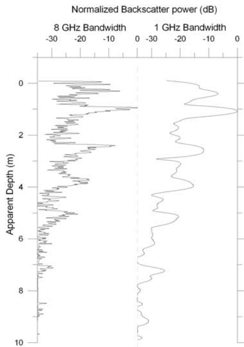
Figure 4. Normalized radar backscatter power return with depth at T12 + 5 km along EGIG (towards summit) in April 2006. Comparison of a measurement at a centre frequency of 13 GHz, bandwidth 8 GHz with a measurement at a centre frequency 13.5 GHz, bandwidth 1 GHz.
