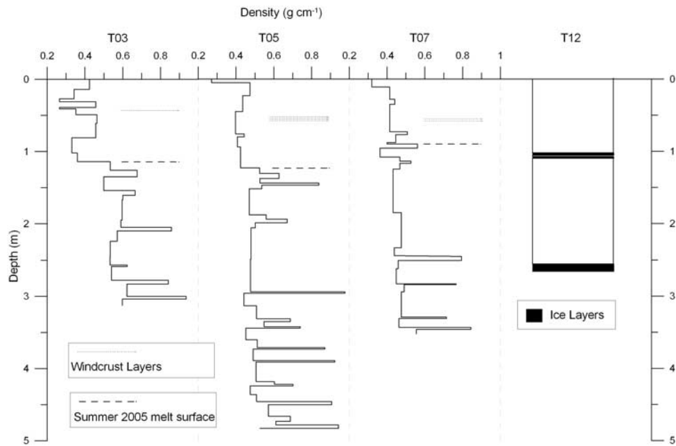
Figure 2. Density – depth profiles from shallow ice cores and pits at T03, T05 and T07, in May 2006. Icy windcrust layers and the summer 2005 melt surface are marked. Ice layers logged in a pit 10 m from T12 in April 2006 are shown.
