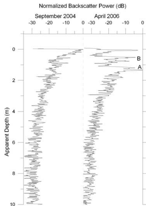
Figure 1. Normalized radar backscatter power return with depth at T05 in September 2004 and April 2006. Centre frequency 13 GHz, bandwidth 8 GHz. The 2005 end of summer surface is marked A. Strong reflectors, believed to be icy windcrust layers, are marked B.
