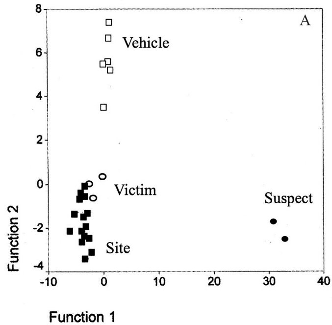
Figure 7 Canonical Discriminant Function plots of chemical analysis by AAS/Dionex (7A) and ICP-MS (7B)
