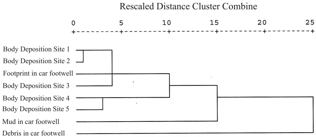
Figure 2 Hierarchical cluster analysis of AAS/Dionex analysis of samples taken from Case Study 1
