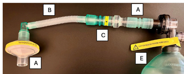
Figure 2. Close up of the LVR bag circuit.
