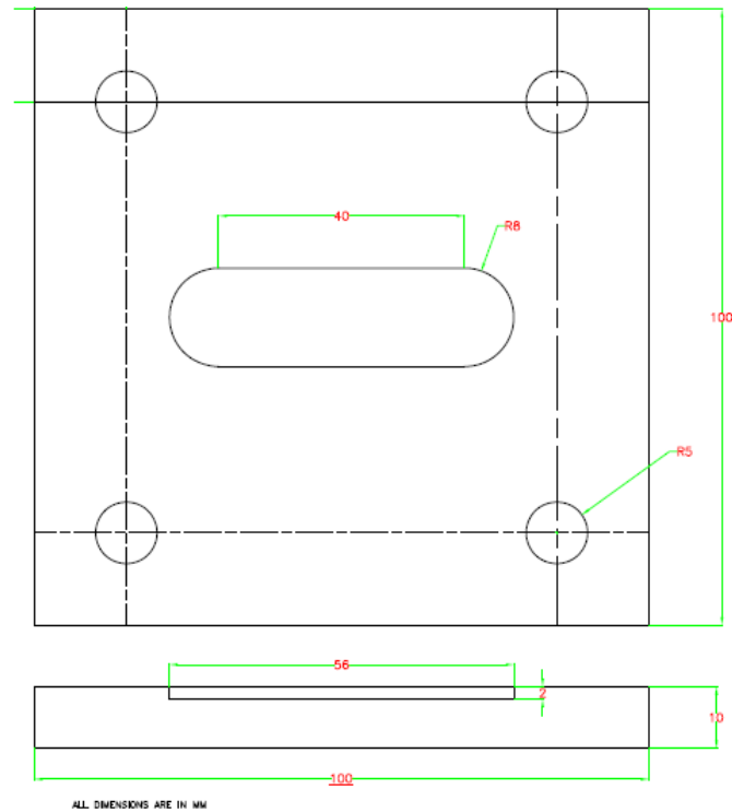
Figure 7: Part-drawing – Milling
