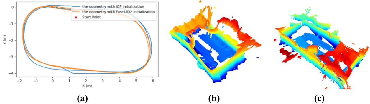
Figure 2: (a) the poses from ICP and Fast-LIO, (b) the dense map with ICP as the front end, and (c) the dense map with Fast-LIO as the front end.
