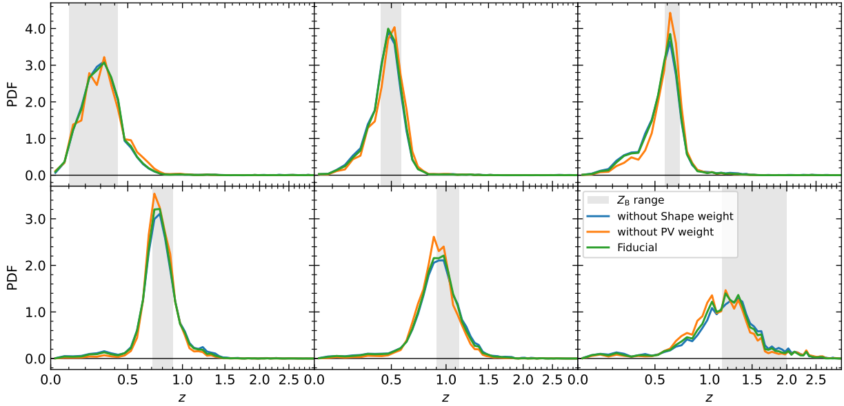
Fig. 12. Estimated redshift distributions from the SOM method, for different analysis choices. Results are highly consistent, except when switching between use or non-use of the prior volume weighting. However, as described in Sect. 4.3, this difference is shown to be reflected in an increased bias for the non-prior-weighted distributions.
