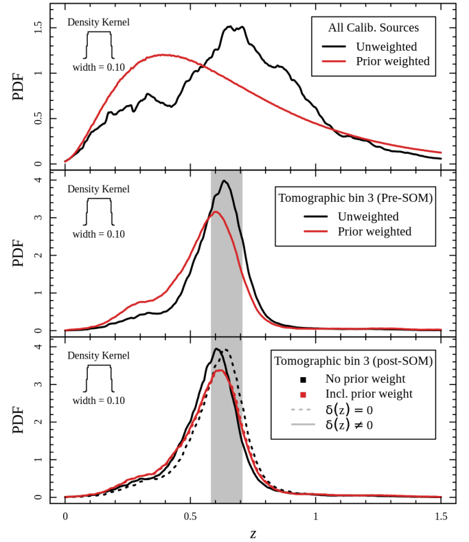
Fig. 6. Impact of prior-volume weights on the (pre-SOM) N(z) of the full spectroscopic compilation (upper panel), and on those galaxies in the compilation that end up in tomographic bin three both prior to the SOM re-weighting (middle panel) and after the SOM re-weighting (bottom panel). The systematic effect that the prior weight imparts on the tomographic bin is particularly clear prior to re-weighting by the SOM to match the wide-field sample but is somewhat diluted by the SOM re-weighting process. Nonetheless, there is a residual difference after the SOM re-weighting in the bottom panel. This difference is exacerbated if one does not have high quality image simulations to calibrate the underlying N(z) bias (dashed lines in the bottom figure; discussed further in Sect. 6), as the non-prior weighted N(z) estimate contains a significant systematic bias ( \langle \delta z \rangle \approx 0.03 ), whereas the prior weighted N(z) estimate has no bias ( \langle \delta z \rangle \approx 0.004 ).
