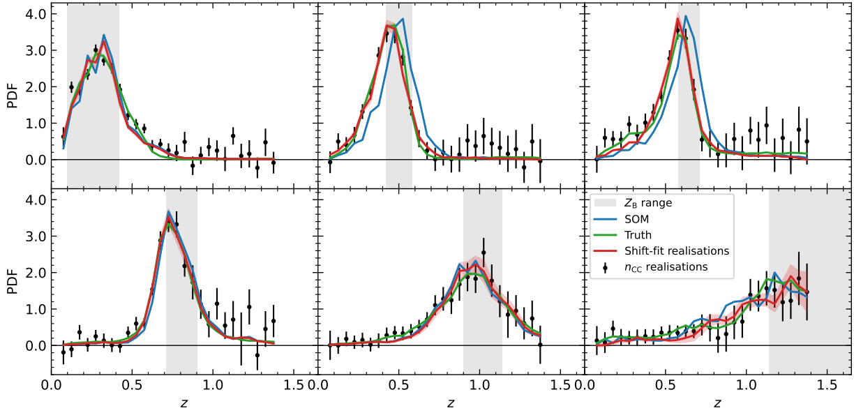
Fig. 10. Comparison of the ensemble of MICE2 realisations and their best-fit solutions when using the SOM redshift distributions as model for the shift-fit. The black data points indicate the mean and standard deviation (encapsulating the added intrinsic scatter) of the CC measurement realisations, the green and blue lines represent the true and SOM redshift distributions, respectively. The red line and shaded area (median and 68% confidence interval) is the N_{\text{SOM}}(z) after applying the shift-fit parameter value in each realisation.
