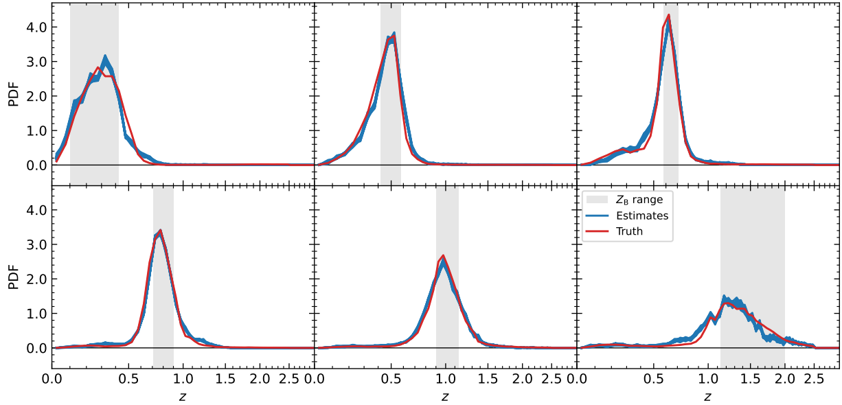
Fig. 9. Redshift distributions for the fiducial SOM calibration methodology, computed using the SKiLLS simulations. The ensemble of blue polygons show the N(z) constructed with different realisations of the calibration sample. Redshift distributions include the new gold-weighting for the wide-field sample, and prior volume weighting and shape-measurement weights for the calibration samples.
