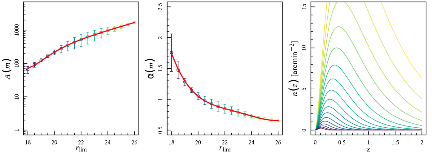
Fig. 5. Model parameters and the resulting analytic N(z) for samples defined as magnitude-limited (in the r band) from our noiseless SURFS+Shark light cone. The left and centre panels show the free parameters from Eq. (2), as a function of the r -band magnitude limit, including polynomial fits. The right panel shows the analytically estimated N(z) for each of the models parameters in the other two panels.
