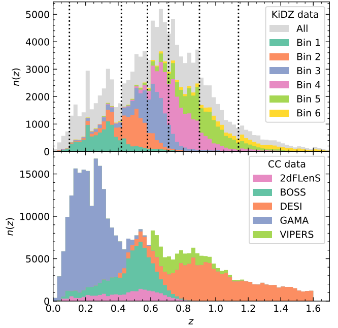
Fig. 1. Redshift distribution of the calibration data used for KiDS-Legacy. The top panel displays the full KiDZ data in grey and the proportion of it that enters each tomographic bin after calibrating the fiducial SOM, shown as a stacked histogram. The bin edges are indicated by the vertical dashed lines. The bottom panel shows the spectroscopic surveys used as calibration samples for the clustering redshift measurements (also stacked).
