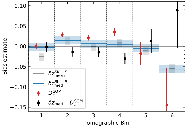
Fig. 14. Comparison of the shift parameters obtained from the KiDS-Legacy data and the SOM bias obtained from SKiLLS. The short grey and blue lines indicate the bias in the mean and median SOM redshift, the red data points the shift-fit parameters D_z when fitting CC measurements with the N_{\text{SOM}}(z) . The black data points represent the difference between the empirical median SOM bias estimate and the shift-fit parameter.
