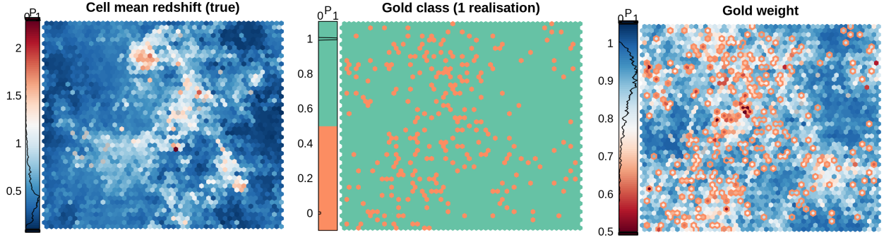
Fig. 3. Comparison between gold-class and gold-weight definitions. Here, a SOM trained on tomographic bin one in our SKiLLS simulation is coloured by the true mean redshift of each cell ( left ), the gold-class definition of each cell under a single realisation ( centre ), and the gold weight of each cell after ten realisations. In the gold-weight panel, the cells, which are assigned a (highly stochastic) zero gold class in our single realisation, are highlighted with an orange border. These cells are assigned a wide range of final gold-weights, highlighting the stochasticity of the gold-class definition and the superiority of the gold-weights. In each colour bar, the PDF of cell values is shown.
