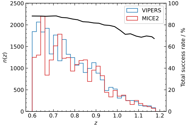
Fig. A.3. Comparison of the VIPERS redshifts distribution (in blue) in the range 0.6 \leq z < 1.18 and MICE2 (in red) after applying the colour and magnitude cuts, and the empirical incompleteness sampling, indicated by the total success rate (black line).
