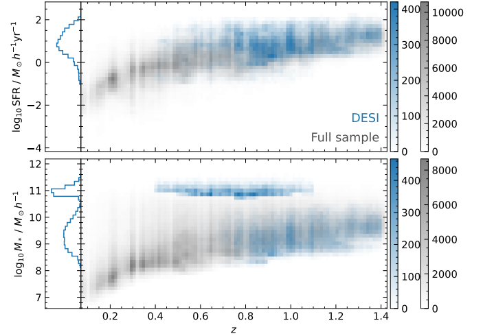
Fig. A.1. Comparison of the star-formation rate (top) and the stellar mass (bottom) for the full MICE simulation (grey) and our simulated DESI LRG and ELG samples (blue) as a function of redshift. The data is selected from a 44 \text{ deg}^2 patch of MICE2. The lower panel clearly shows the separation of the ELG from the LRG sample, which is selected based on stellar mass.
