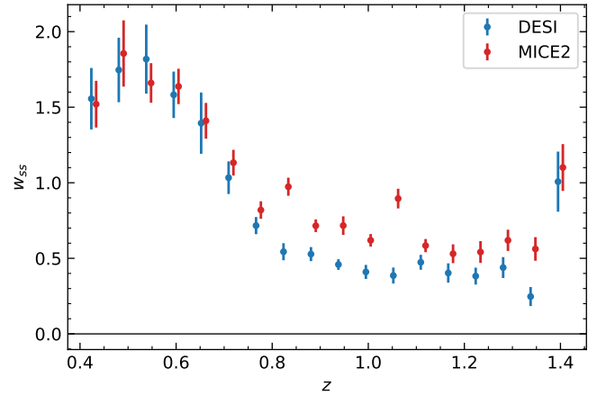
Fig. A.2. Auto-correlation amplitude measured between 100 and 1000 kpc for DESI (in blue) and MICE2 (in red).
