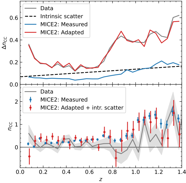
Fig. 8. One realisation of the CC measurements from MICE2 in the sixth tomographic bin after noise adaptation (Sect. 5.3) and the addition of intrinsic scatter (Sect. 5.4). The top panel compares only the uncertainties of N_{CC}(z) from the data (grey) and MICE2 before (blue) and after adaptation (red). The dashed black line indicates the fitted intrinsic scatter from the measurements on the data ( f = 0.14 \pm 0.04 ; see Eq. 6). The bottom panel shows the measured N_{CC}(z) from MICE2 (blue points) compared to the data (grey line). The red data points represent the MICE2 measurements after adapting the noise (up-scaling errors and perturbing values) and adding the intrinsic scatter (only perturbing values) obtained from the data.
