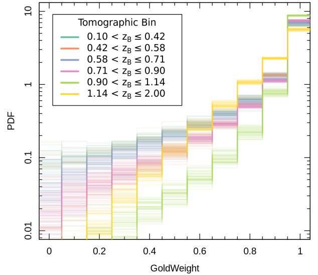
Fig. 4. Distributions of gold weight per tomographic bin for our fiducial SKiLLS simulations. Individual lines show the scatter in the gold-weight PDFs under different realisations of our spectroscopic calibration samples. The tomographic bins show qualitatively similar behaviour: many sources are consistently classed as gold under all realisations of the SOM ( w_{\text{gold}} = 1 ), and very few sources are consistently classed as not-gold under all realisations ( w_{\text{gold}} = 0 ).
