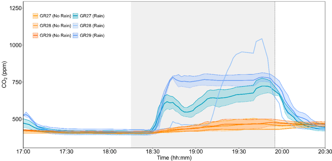
Fig. 6. Spatially averaged CO 2 over time in three naturally ventilated marquees (GR27, GR28, GR29) on a day with and without rain. Solid lines indicate the spatial average for each zone, with the shading indicating the minimum and maximum values, where there was more than one sensor in the space. The shaded section shows occupied time from 18:15 to 19:50.
