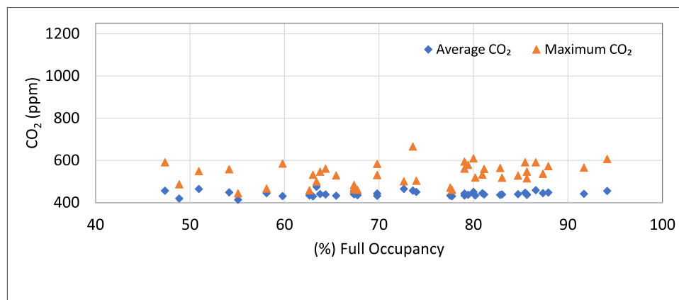
Fig. 8. Spatiotemporal mean and point-in-time and space maximum CO 2 concentration and varying occupancy in the graduation marquee (LO) at all 41 events.
