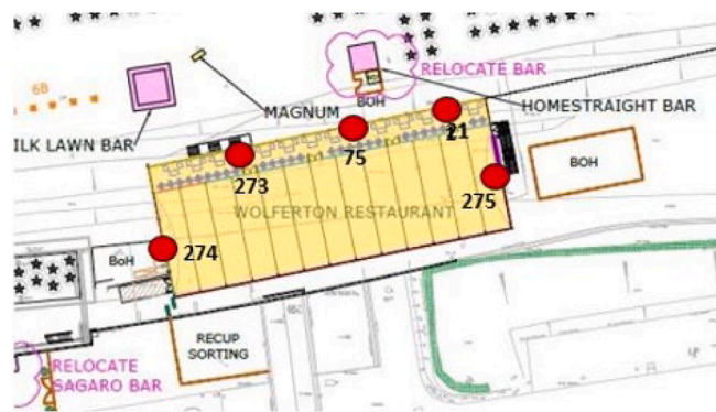
Fig. 15. RA5 marquee at ascot racecourse. Red dots indicate the location of a CO 2 sensor.
