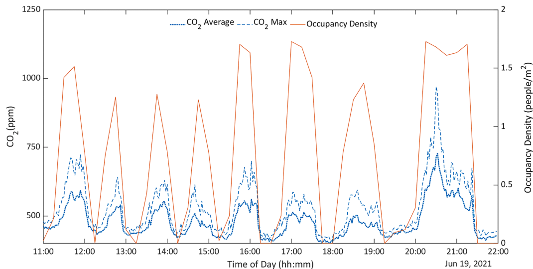
Fig. 9. Occupancy density (calculated from CCTV imagery), spatial CO 2 average and spatial CO 2 maximum as a function of time in the middle zone at Download Festival (19 June).
