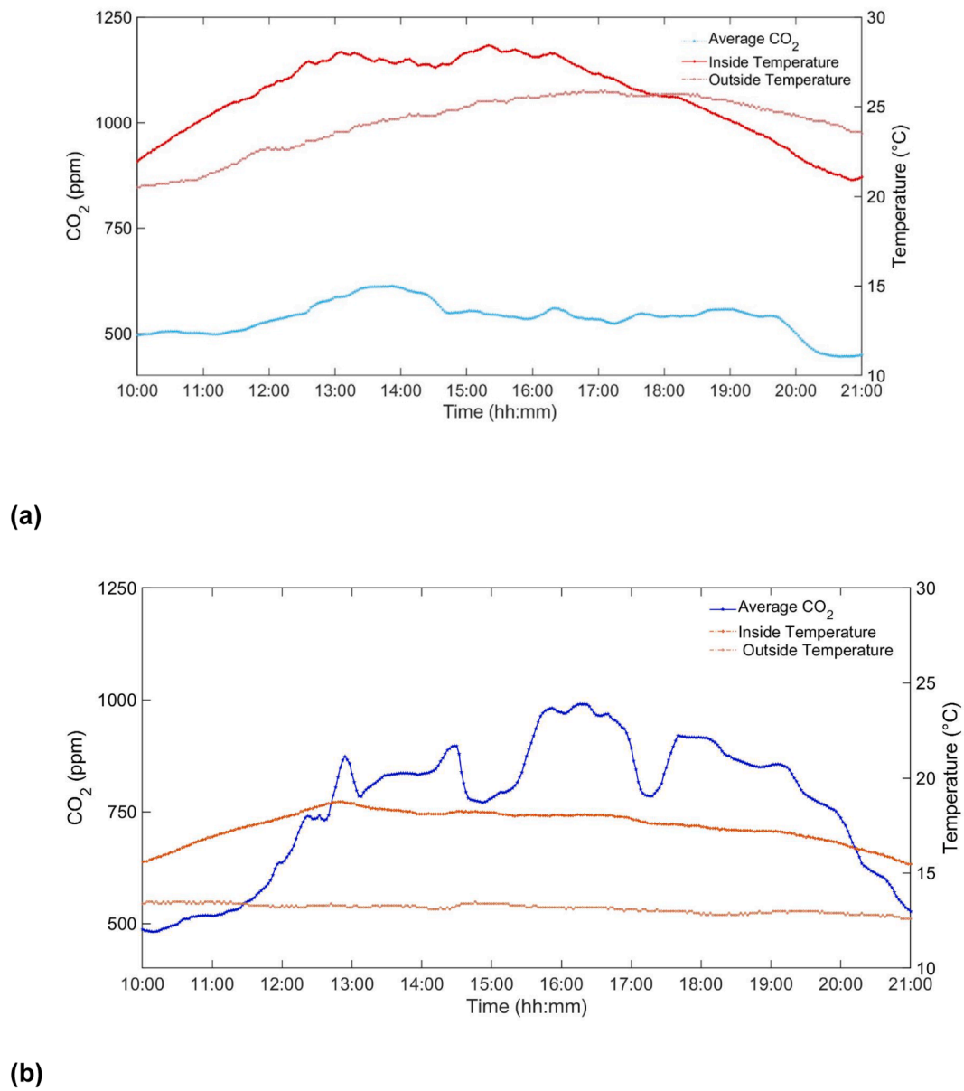
Fig. 7. Outdoor temperature, indoor temperature, and spatially averaged indoor CO 2 concentration over time in a mechanically ventilated marquee (RA5) on (a) a hot weather day and (b) a cool weather day.
