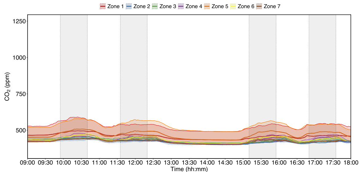
Fig. 11. CO 2 concentration profile versus time of day in the graduation ceremony marquee on the day with the highest occupancy (486 people; 0.32 people/m 2 ). Solid lines indicate the spatial average for each zone, with the shading indicating the minimum and maximum values. Greyed sections indicate the ceremony times (four ceremonies on this day, usually five).
