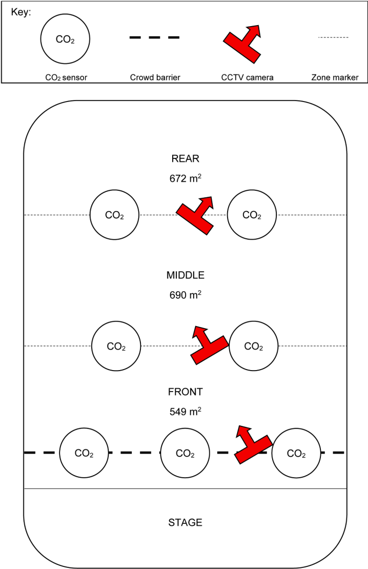
Fig. 16. Floorplan, sensor locations, and video camera positions in the semi-outdoor music festival tent.
