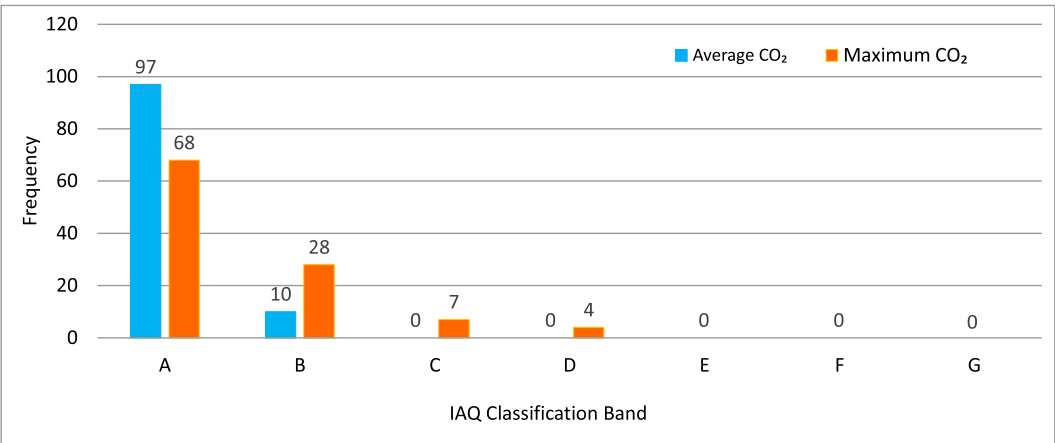
Fig. 4. Spatiotemporal mean average and maximum CO 2 in all semi-outdoor spaces monitored over all events, aggregated by air quality bands.
