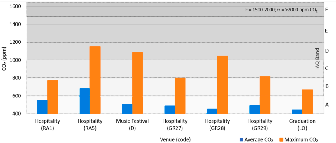
Fig. 5. Spatiotemporal mean and maximum air quality classification bands for semi-outdoor spaces across all 78 events.
