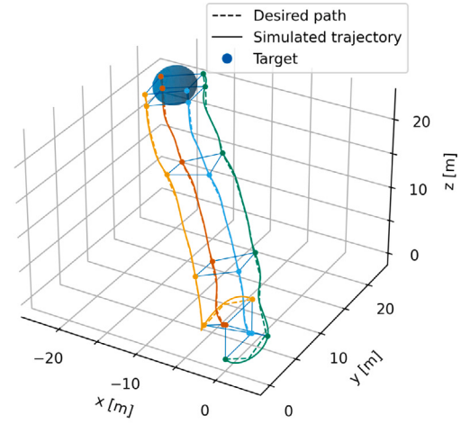
(b) Tracking the target \mathbf{t} = (-20, 20, 20)
