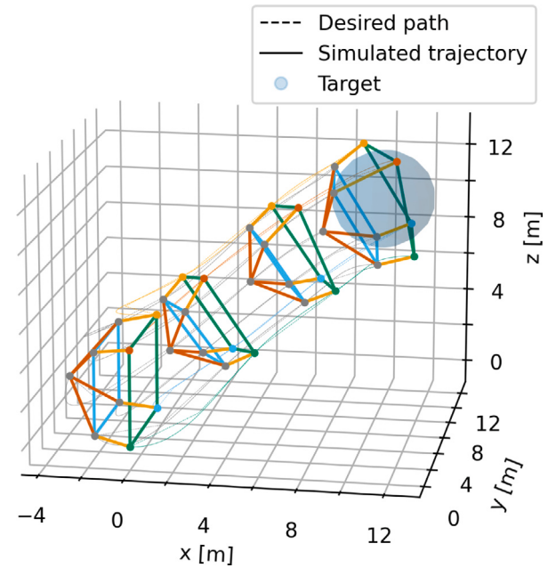
Fig. 8. The simulation of a hemispherical formation surrounding a remote target. The leader UAVs are represented as coloured markers and the followers are in grey. The formation covers the target whilst maintaining its formation. Only the leader UAVs require path planning.
