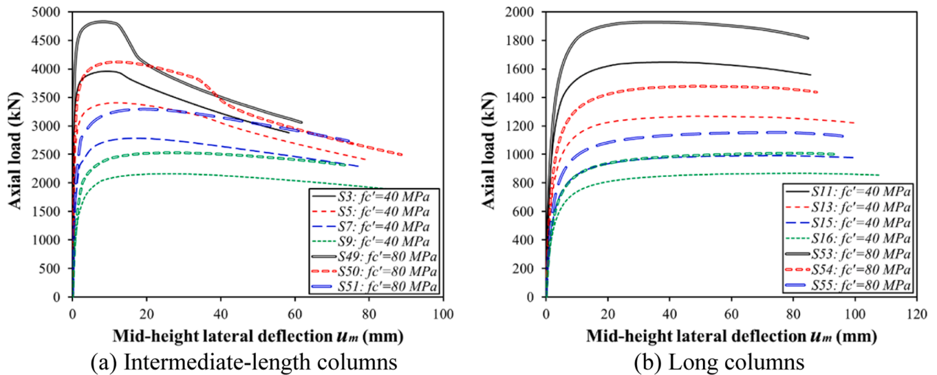
Fig. 23. Effect of concrete strength on the axial load-lateral deflection responses.
