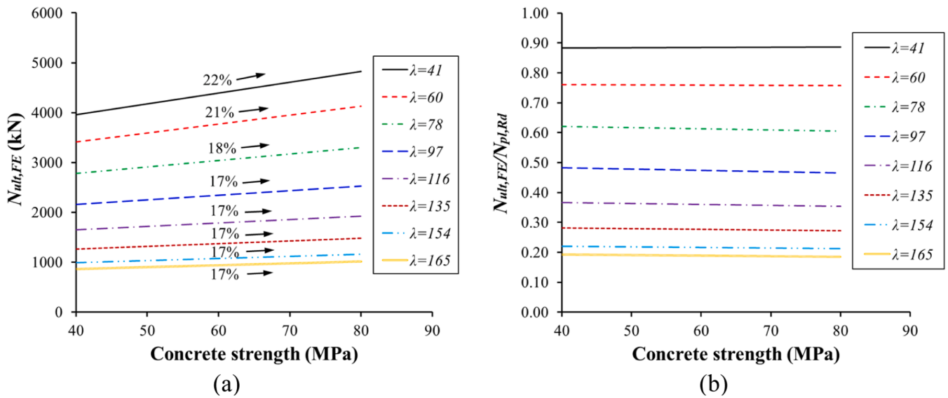
Fig. 22. Effect of concrete strength on: (a) ultimate and (b) normalized strengths.
