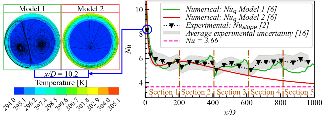
Fig. 6: Experimental [2] and numerical [6] local Nusselt numbers with temperature contours and velocity streamlines at x/D = 10.2 for Models 1 (green outlines) and 2 (red outlines) at an inlet Reynolds number of 902 and an average wall temperature of 29.1^{\circ}\text{C} .
