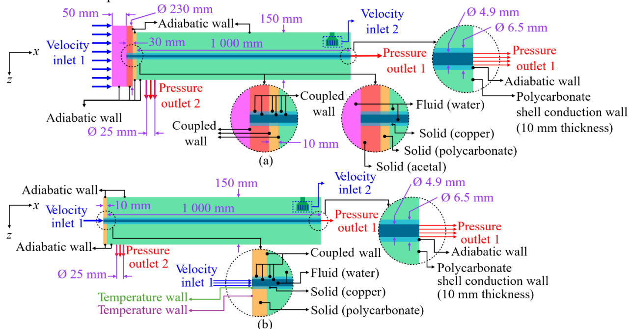
Fig. 2: Top view of (a) computational domain 1 and (b) computational domain 2 for Model 1. Adapted from [6].
