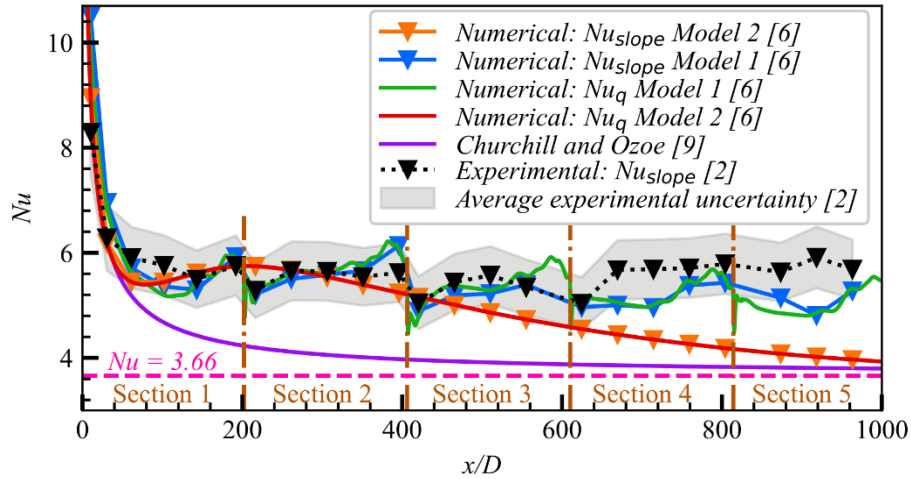
Fig. 4: Experimental [2] and numerical [6] local Nusselt numbers at an inlet Reynolds number of 902 and an average wall temperature of 29.1°C.
