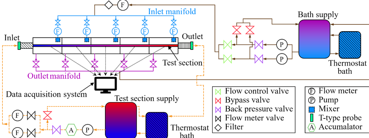
Fig. 1: Schematic of the experimental setup showing two flow loops. The first (dotted orange lines) facilitated flow through the copper tube test section, while the second (solid brown lines) circulated flow through five water bath sections. Adapted from [2].
