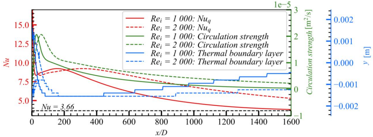
Fig. 5: Numerical local Nusselt numbers (red), circulation strength (green), and thermal boundary layer thicknesses (blue) of Model 2 for an inlet Reynolds number of 1 000 (solid lines) and 2 000 (dashed lines) at an initial wall-fluid temperature difference of 30°C. Adapted from [6].
