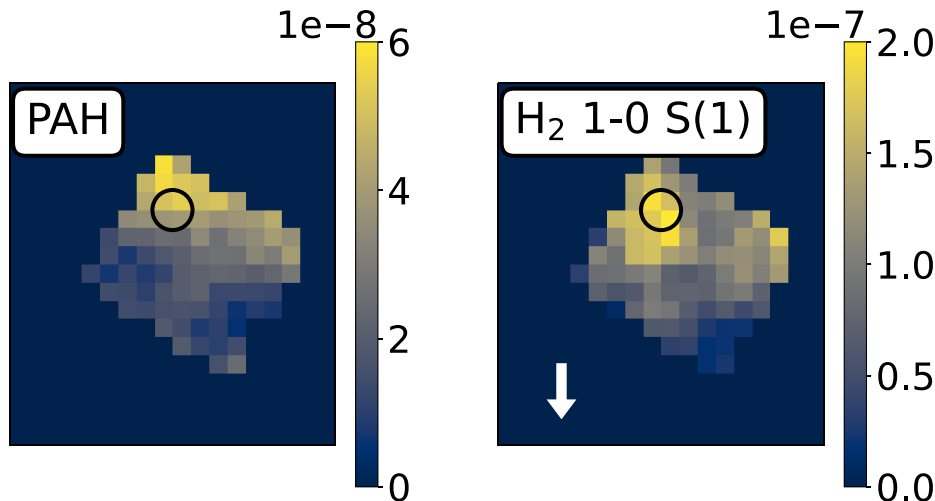
Figure 9. The morphology of the 3.3 \mu\text{m} PAH emission (left), and the \text{H}_2 1–0 S(1) emission (right) for the north region. The black circle indicates the location of the peak \text{H}_2 1–0 S(1) emission. The arrow in the right panel indicates the approximate direction of the central source. The data are regridded to 2 pixels by 2 pixels, in order to reduce noise. The integrated surface brightness displayed on the colourbar is in units of \text{W m}^{-2} \text{sr}^{-1} . The maps on a pixel scale of 0.1 arcsec are shown in Fig. E1.
