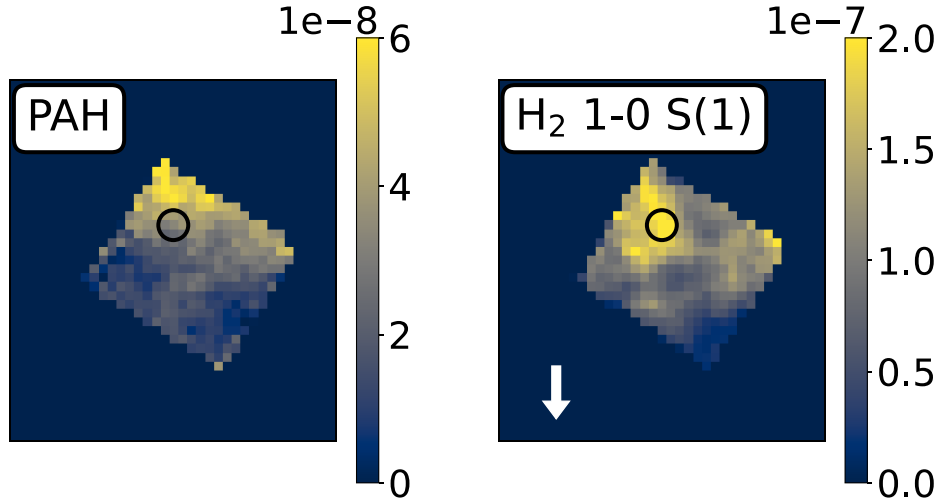
Figure E1. The morphology of the 3.3\ \mu\text{m} PAH emission (left) and the \text{H}_2\ 1-0\ \text{S}(1) emission (right) for the north region. The black circle indicates the location of the peak \text{H}_2\ 1-0\ \text{S}(1) emission. The arrow in the right panel indicates the approximate direction of the central source. This map is in the original pixel scale of 0.1\ \text{arcsec} spaxels. The integrated surface brightness displayed on the colourbar is in units of \text{W m}^{-2}\ \text{sr}^{-1} .
