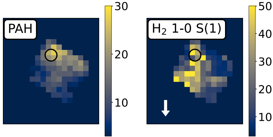
Figure E2. The signal-to-noise ratio maps corresponding to Fig. 9 (i.e. when the data are re-binned to a 2 \times 2 grid). The black circle indicates the location of the peak \text{H}_2\ 1-0\ \text{S}(1) emission. The arrow in the right panel indicates the approximate direction of the central source.
