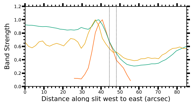
Figure 10. The integrated surface brightness of the Spitzer /IRS SL1 11.2 \mu\text{m} PAH emission (orange, in units of \text{W m}^{-2} \text{sr}^{-1} ), the NIRC Cam F335M/F300M ratio (yellow, in units of \text{MJy sr}^{-1} ), and the MIRI F1130W/F1000W ratio (green, in units of \text{MJy sr}^{-1} ) along the Spitzer /IRS SL1 slit shown in Fig. 1. All measurements shown are \geq 3\sigma detections. Each curve is scaled to have a peak band strength of 1. Scaling factors are 7.22 \times 10^{-8} , 2.38, and 1.54, respectively. The vertical dashed lines indicate the location of the JWST north region, as it is contained within the Spitzer /IRS SL1 slit. The aperture ‘ Spitzer /IRS SL1 Peak’ seen in Fig. 1 corresponds to 35–45 arcsec along the slit.
