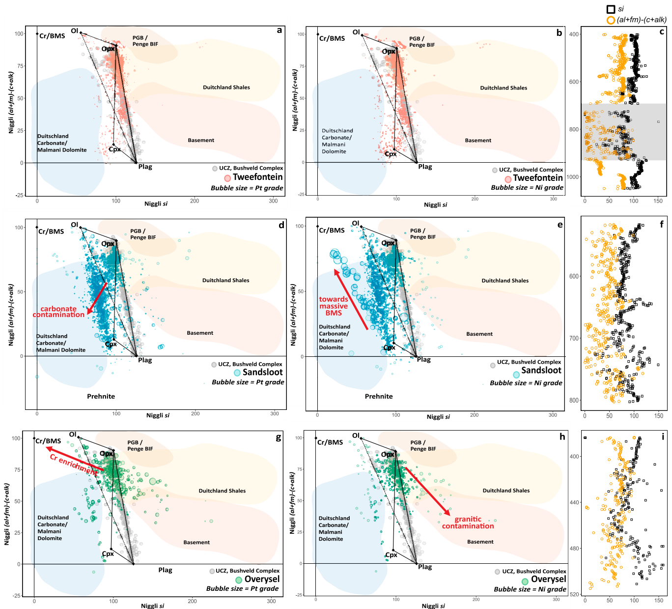
Fig. 5. Niggli (al + fm) - (c + alk) vs si bubble plots for the Platreef at each study location, the UCZ of the western and eastern limbs, Transvaal footwall lithologies and downhole plots for example drillholes. Bubble sizes for the Platreef data are scaled to either Pt (ppm) or Ni (wt%) grades; a-b) Tweefontein Pt and Ni grades respectively. Magmatic units only. No Ni data was available for drillholes TN303 or TN304; c) Downhole Niggli si and (al + fm) - (c + alk) plot for RTN021; d-e) Sandsloot Pt and Ni grades respectively; f) Downhole Niggli si and (al + fm) - (c + alk) plot for SSAA019; g-h) Overysel Pt and Ni grades respectively. i) Downhole Niggli si and (al + fm) - (c + alk) plot for OY1050. An_{80} composition for UCZ plagioclase chosen after McDonald (2024). For lithology logs see Fig. 2. A xenolith raft in RTN021 (shaded grey) is not shown in the bubble plots.
