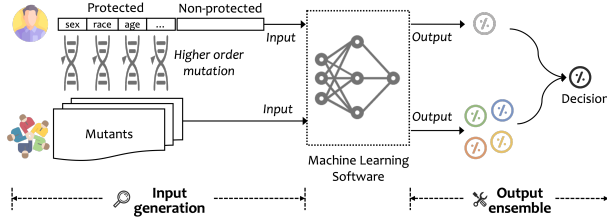
Fig. 1: Overview of FairHOME.
