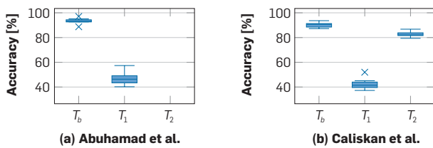
Figure 2. Accuracy of authorship attribution after considering artifacts. The accuracy drops by 48% if unused code is removed from the test set ( T_1 ); After retraining ( T_2 ), the average accuracy still drops by 6% and 7%.
