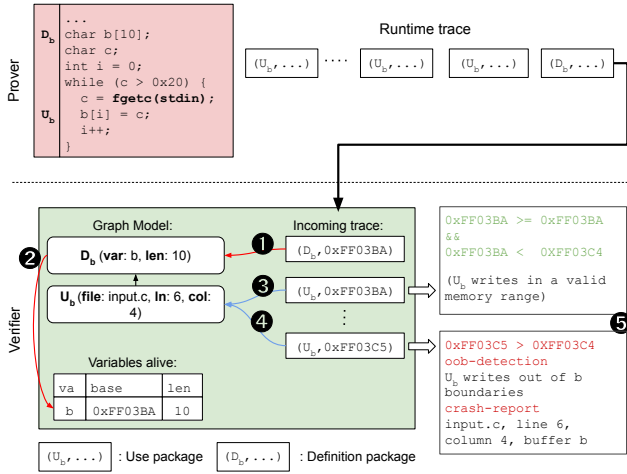
Figure 2: EMBEDWATCH Protocol. The prover sends a stream of Use and Definitions that represents the variable alive and their use. The Verifier infers the firmware state from the runtime trace and the Use-Def graph. The Use-Def graph reduces the size of the runtime trace in two ways (1) it avoids transmitting static information (e.g., the buffer b length), and (2) it minimizes the instrumentation points (the only possible out-of-bound use is U_b ).
