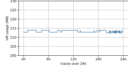
Figure 3: Virtual Memory (VM) allocated by the Verifier after 24h of interaction with a firmware.
