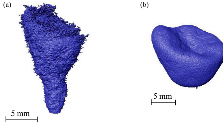
Fig. 6. 3D structure of gas morphology: (a) Morphological characteristics at point J and (b) morphological characteristics at point K.
