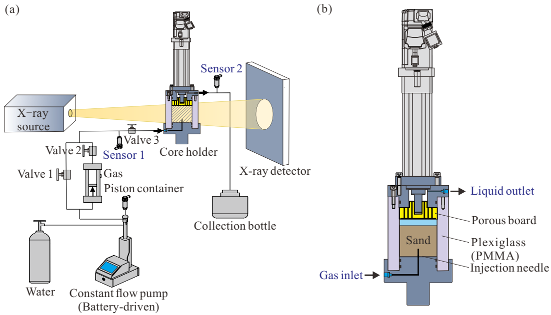
Fig. 2. Sketch of test apparatus: (a) Experimental system and (b) structure of the core holder.
