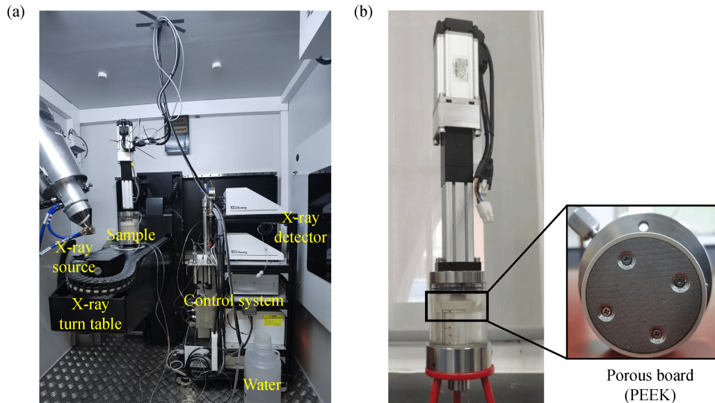
Fig. 3. Experimental device: (a) Configuration of the micro-ct scanner and (b) core holder and porous board.
