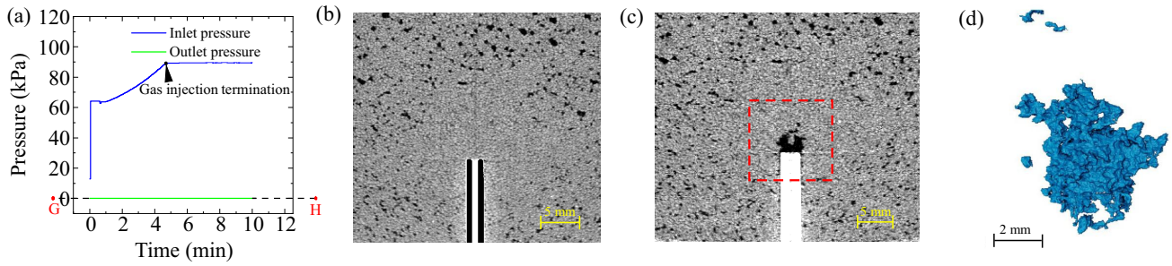
Fig. 7. Independent experiment for verifying internal conditions during gas accumulation period: (a) Gas pressure curve, (b) 2D slice of the state of point G, (c) 2D slice of the state of point H and (d) 3D structure of the red dotted box in (c).
