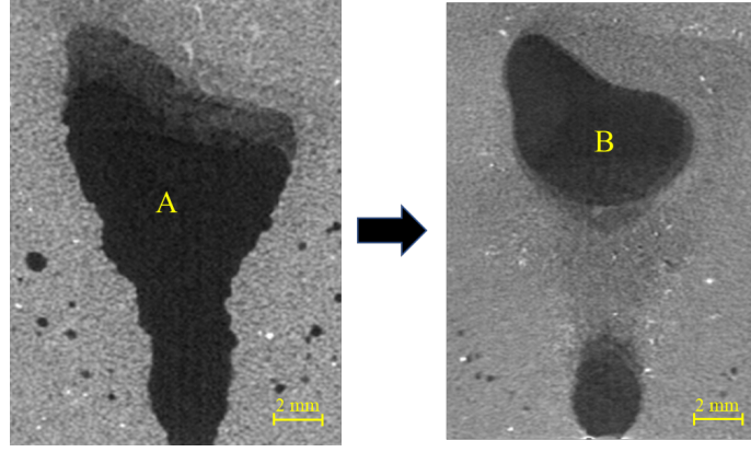
Fig. 12. Visualization of healing mechanism through X-ray image (From A to B). The black areas represent gas.
