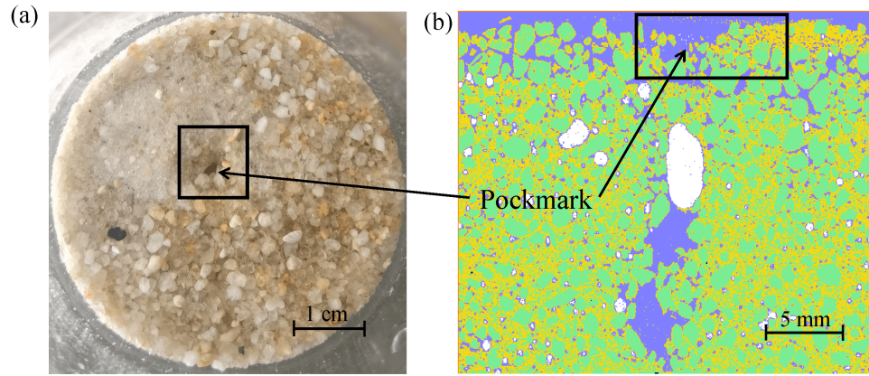
Fig. 9. Gas injection experiment result for the particle size range of 0.075 to 1.40 mm: (a) A photo of sediment surface and (b) the internal CT image. White stands for gas, blue for water, green for sand, and yellow represents a mixture of fine sand and water. The black boxes in (a) and (b) represent pockmarks formed after gas injection.
