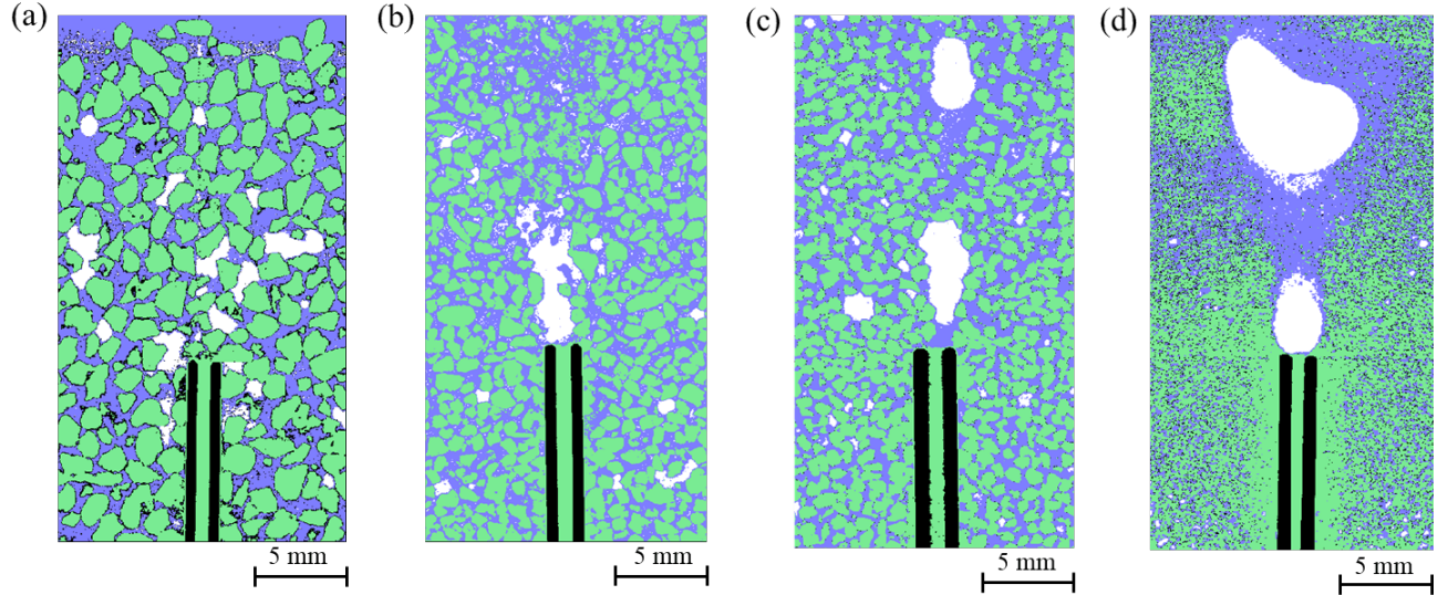
Fig. 8. Gas migration patterns at different particle sizes: (a) d = 1.18-1.40 mm, (b) d = 0.60-1.18 mm, (c) d = 0.30-0.60 mm and (d) d = 0.15-0.30 mm. Gas, water and sand particles are marked in white, blue and green, respectively.
