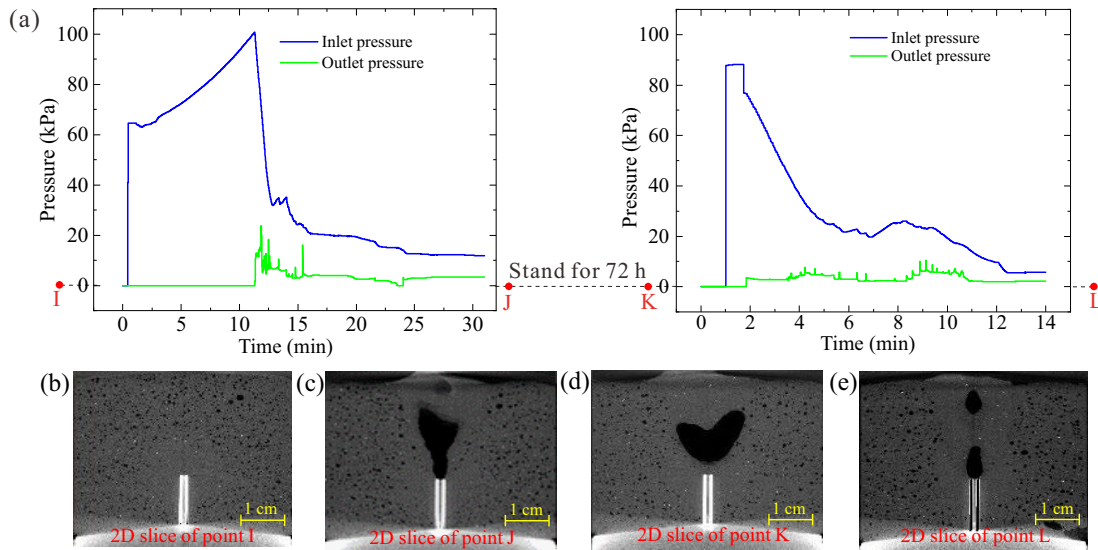
Fig. 5. Results of the complete gas migration experiment combined with CT 3D reconstruction: (a) Gas pressure curve and (b)-(e) the 2D slices of points I, J, K, L respectively represent the sediment states before and after the first gas migration and those before and after the secondary gas migration.
