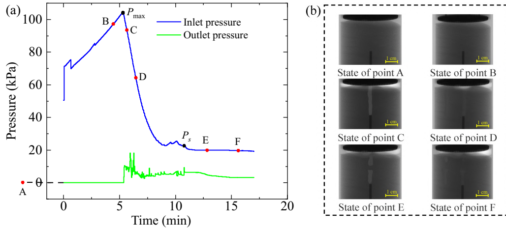
Fig. 4. Results of the gas injection experiment: (a) The gas pressure curve and (b) 2D X-ray projections at points A-F.
