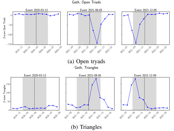
Fig. 9: Go-ethereum repository. The black vertical line marks the event, while the grey shaded area represents the three months before and after the event. The blue line shows the trend of the Z-score for the triadic motifs over time
