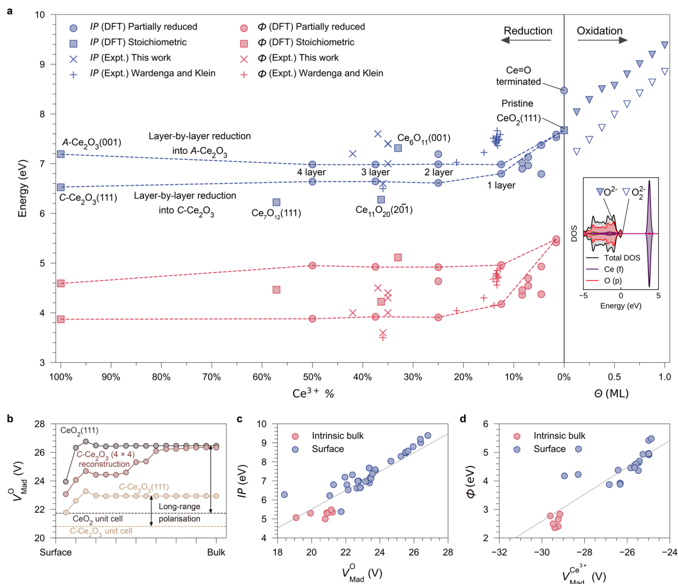
Figure 4. Environmental modulation of IP and \Phi of cerium oxides and its relevance to electrostatics. (a) Variation of IP and \Phi in (111)-terminated \text{CeO}_2 in different reduction and oxidation environments from DFT calculations and experimental measurements in this work as well as by Wardenga and Klein. 23 The inset is the DOS of the 1-ML-peroxide-covered (111) surface, showing a split valence band due to lattice \text{O}^{2-} (filled triangles) and surface \text{O}_2^{2-} (empty triangles). (b) Layer-by-layer distribution of V_{\text{Mad}}^{\text{O}} penetrating from the surface layer to the bulk region under pristine \text{CeO}_2 (111), partially reduced \text{C-Ce}_2\text{O}_3 ( 4 \times 4 ) reconstruction on \text{CeO}_2 (111), and fully reduced \text{C-Ce}_2\text{O}_3 (111). Dashed lines indicate the V_{\text{Mad}}^{\text{O}} calculated in periodic unit cells of \text{CeO}_2 and \text{C-Ce}_2\text{O}_3 , respectively, which are the pure bulk contributions to the electrostatics that exclude surface effects. The double arrows highlight the differences in V_{\text{Mad}}^{\text{O}} calculated in periodic unit cells and in the bulk region under the (111) surface of \text{CeO}_2 and \text{C-Ce}_2\text{O}_3 , which originate from long-range surface polarization. (c) Relationship between the IP of reduced ceria with the lowest V_{\text{Mad}}^{\text{O}} . (d) Relationship between the \Phi of reduced ceria with the lowest V_{\text{Mad}}^{\text{Ce}^{3+}} .
