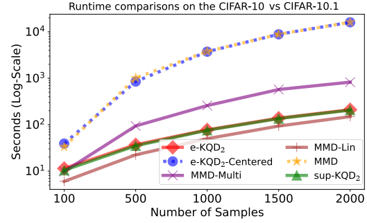
Figure 4: Comparing the time (in seconds) required to complete the CIFAR-10 vs. CIFAR-10.1 experiment, plotted on a logarithmic scale. A shorter time indicates a faster algorithm. These results align with our complexity analysis.
