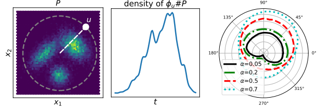
Figure 1: Illustration of bivariate quantiles. Left: Bivariate distribution P . Center: Density of the projection of P onto direction u on the unit circle, with \phi_u(x) = \langle u, x \rangle . Right: different quantiles for all possible directions u .
