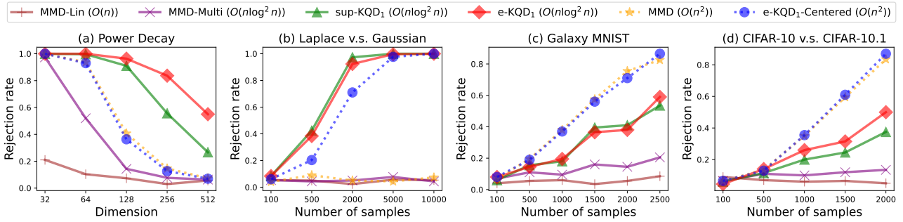
Figure 6: The experiments in Figure 3 repeated for p = 1 . Experimental results comparing our proposed methods with baseline approaches. A higher rejection rate indicates better performance in distinguishing between distributions. Same as for p = 2 , quadratic-time quantile-based estimators perform comparably to quadratic-time MMD estimators, while near-linear time quantile-based estimators often outperform their MMD-based counterparts.
