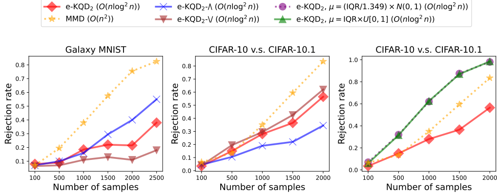
Figure 7: Gaussian KQD test power under different weighting measures. Left, middle : Varying measure \nu : down-weighting ( \setminus ) extremes boosts power on Galaxy MNIST, while up-weighting ( \setminus ) them helps on CIFAR. Uniform weighting remains a strong default, with optimal \nu depending on the dataset. Right : Varying measure \xi : using an IQR-scaled Gaussian or uniform default reference measure \xi both outperform MMD—indicating potential advantage of a "default" \xi over the problem-based \xi = (P_n + Q_n)/2 .
