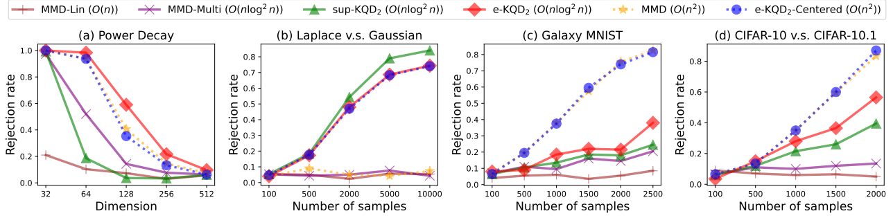
Figure 3: Experimental results comparing our proposed methods with baseline approaches. Methods represented by dotted lines exhibit quadratic complexity for a single computation of the test statistic, while the remaining methods achieve near-linear or linear computational efficiency. A higher rejection rate indicates better performance in distinguishing between distributions. Overall, quadratic-time quantile-based estimators perform comparably to quadratic-time MMD estimators, while near-linear time quantile-based estimators often outperform their MMD-based counterparts.
