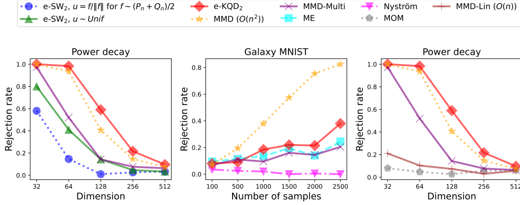
Figure 8: All methods are cost \mathcal{O}(n \log^2 n) unless specified otherwise. Left: Gaussian KQD compared with sliced Wasserstein with uniform or data-driven directions, on the power decay problem. Sliced Wasserstein fall well below KQD—consistent with their equivalence to KQD using a less expressive linear kernel. Middle: Comparison with alternative approximate KME methods, at matching cost. ME matches MMD-multi power, while Nyström-MMD suffers high Type II error. Right: Comparison with Median-of-Means (MOM) KME approximation, at matching cost. MOM is primarily a robustness-enforcing method, not a cheap-approximation method, and doesn't perform well at set cost of \mathcal{O}(n \log^2 n) .
