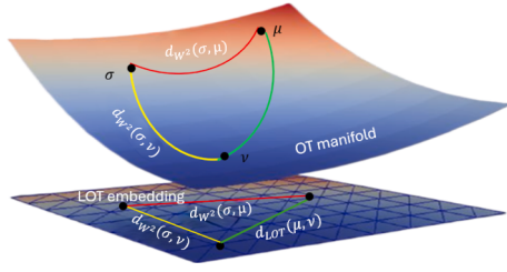
Fig. 1. The Linear Wasserstein framework embeds measures in the tangent space of a fixed reference \sigma . As a consequence, the Euclidean distance between the non-negative measures \mu and \nu is an approximation for the 2-Wasserstein distance d_{W^2}(\mu, \nu) . This figure is computed using ParaView.
