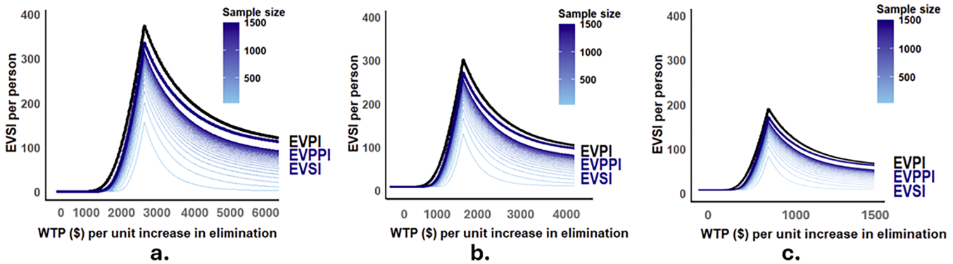
Fig. 5. EVSI estimated using the Moment Matching method, for three baseline prevalence ranges: (a) 5–10 % with WTP_{DALY} = \$500 , (b) 10–20 % with WTP_{DALY} = \$2500 , and (c) 20–30 % with WTP_{DALY} = \$5000 by varying the number of iterations (sample size) used in the transmission model (equivalently, the epidemiological outcomes used as inputs in the health-economic decision model). The EVSI quantifies the value of reducing uncertainty when lowering the stopping threshold for TAS to < 0.5\% mf prevalence in a sample of adults. Estimates are shown across a range of WTP_{Elimination} , assuming 65 % MDA coverage.
