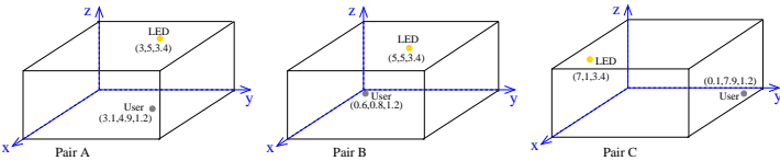
Fig. 5: Room topology and three LED-User pairs.
