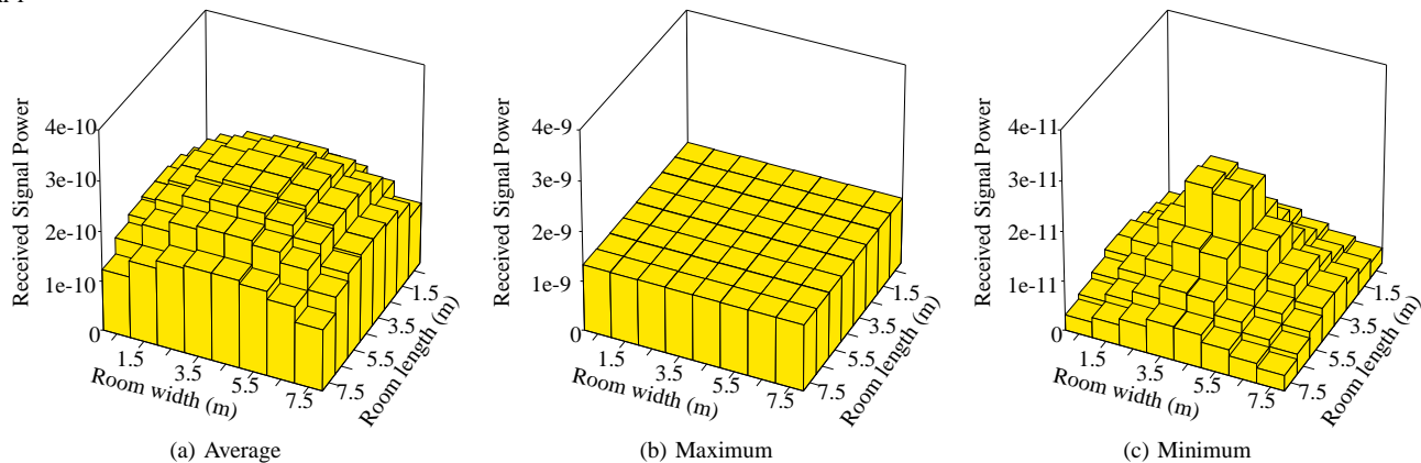
Fig. 16: Illumination functionality : Received signal power in LoS scenario, where we have P_t = -20\text{dBm} . The subfigures are average, maximum and minimum received signal powers of all LED-User pairs in each 1 \times 1 \text{ m}^2 area.
