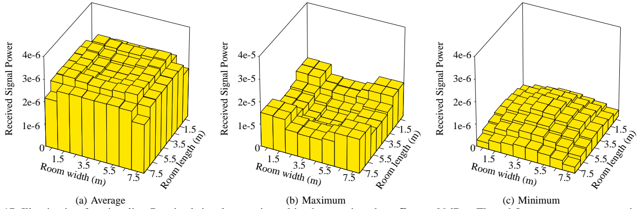
Fig. 17: Illumination functionality : Received signal power in multipath scenario, where P_t = -20\text{dBm} . The subfigures are average, maximum and minimum received signal powers of all LED-User pairs in each 1 \times 1 \text{ m}^2 area.
