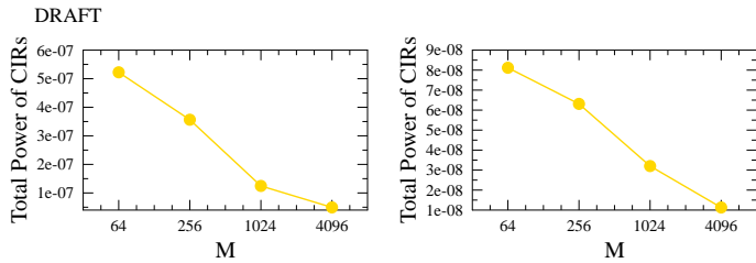
(a) Pair A (b) Pair B Fig. 4: Effect of bandwidth on the total power of CIRs: Total power of CIRs associated with different number of subcarriers M and bandwidth BW = M \cdot SCS , where the transmit power is given by P_t = -20 dBm. The simulation parameters for the multipath scenario are detailed in Sec. VI. The subfigures are plotted for (a) LED-User Pair A, (b) LED-User Pair B.
