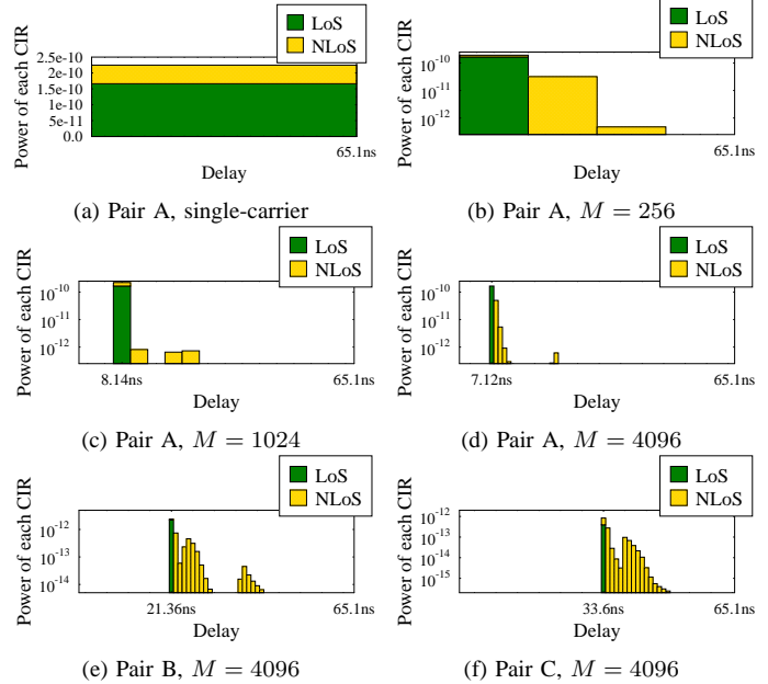
(a) Pair A, single-carrier (b) Pair A, M = 256 (c) Pair A, M = 1024 (d) Pair A, M = 4096 , (e) Pair B with M = 4096 , (f) Pair C with M = 4096 . SCS=240 kHz is fixed. Fig. 6: Power of each CIR for VLPC-DCO-OFDM with different bandwidths BW = M \cdot SCS in multipath scenario. The subfigures are (a) Pair A with single-carrier, (b) Pair A with M = 256 , (c) Pair A with M = 1024 , (d) Pair A with M = 4096 , (e) Pair B with M = 4096 , (f) Pair C with M = 4096 . SCS=240 kHz is fixed.
