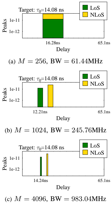
Fig. 2: Effect of bandwidth on CIR: VLPC-DCO-OFDM sensing peaks associated with different number of subcarriers M and bandwidth BW = M \cdot SCS . The coordinates of LED, PD and wall reflection are given by \mathbf{c}_S = [3, 5, 3.4] , \mathbf{c}_D = [1, 2, 1.2] , \mathbf{c}_R = [0, 2, 2] , and their unit normal vectors are \mathbf{n}_S = [0, 0, -1] , \mathbf{c}_D = [0, 0, 1] , \mathbf{c}_R = [1, 0, 0] . The areas of PD and wall reflection are given by A_{PD} = 1\text{cm}^2 and A_{R_1} = 2\text{cm}^2 . The transmit power is given by P_t = -20 dBm. The sensed peaks are obtained based on (16).
