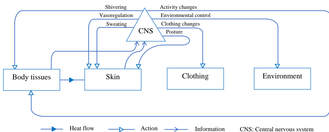
Fig. 1. Thermal comfort as a component of a complex adaptive self-regulating system
