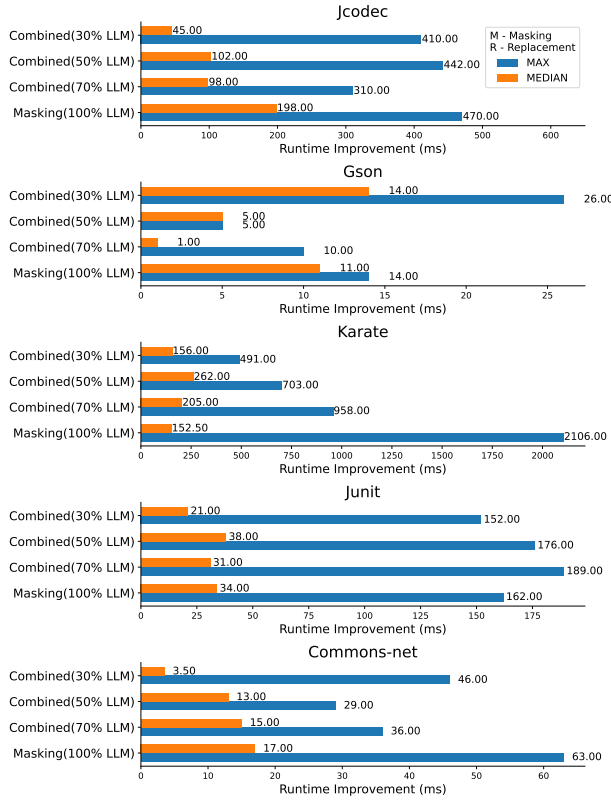
Fig. 6. Local search results for the combined search using the masking mutation and Mistral:7B model, displaying max and median runtime improvements.
