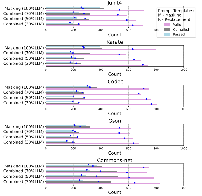
Fig. 5. Random sampling results for the combined search using the masking mutation and Mistral:7B model, showing the number of valid, compiled, and test-passing patches. The blue dot indicates the number of unique patches.
