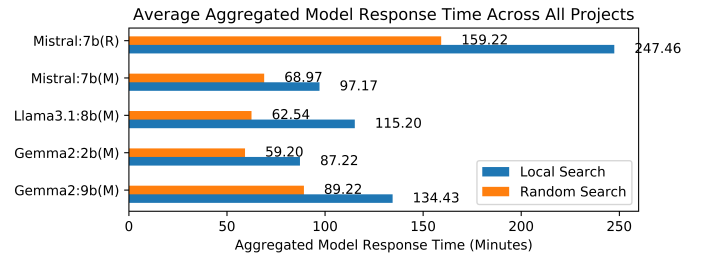
Fig. 4. Avg. model response time across all projects for each model and mutation combination. (M) denotes masking, and (R) replacement mutation.
