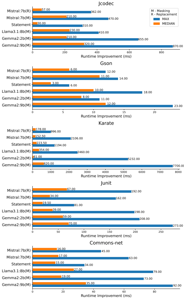
Fig. 3. Local search results for each LLM and project combination, showing the maximum and median runtime improvements. (M) denotes masking mutation results, and (R) denotes replacement mutation results. Statement represents the traditional GI mutations.
