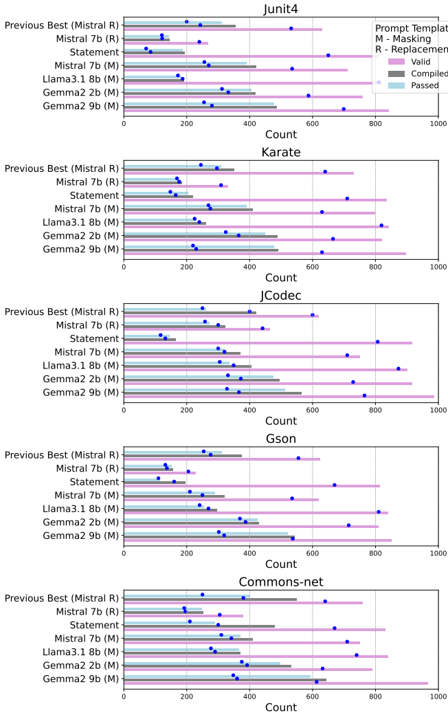
Fig. 2. Random sampling results for each LLM and project combination, illustrating the counts of valid, compiled, and test-passing patches. Blue dots indicate unique patches. (M) denotes the masking mutation, (R) represents the replacement mutation, and Statement refers to traditional GI mutations. “Previous Best (Mistral R)” reflects the results of Mistral:7B from Brownlee et al.’s work [5], while “Mistral:7B (R)” represents the replacement mutation results for Mistral:7B, as recreated in our experimental environment.
