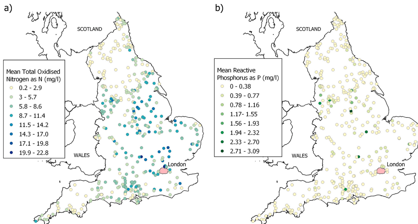
Fig. 1. Mean Total Oxidised Nitrogen (TON) (a) and mean Reactive Phosphorus (RP) (b) for the years 2015–2019 at the monitoring stations initially selected based on minimum data availability, and after ensuring that the monitoring stations' catchments did not overlap. For TON n = 404 , for RP n = 383 .
