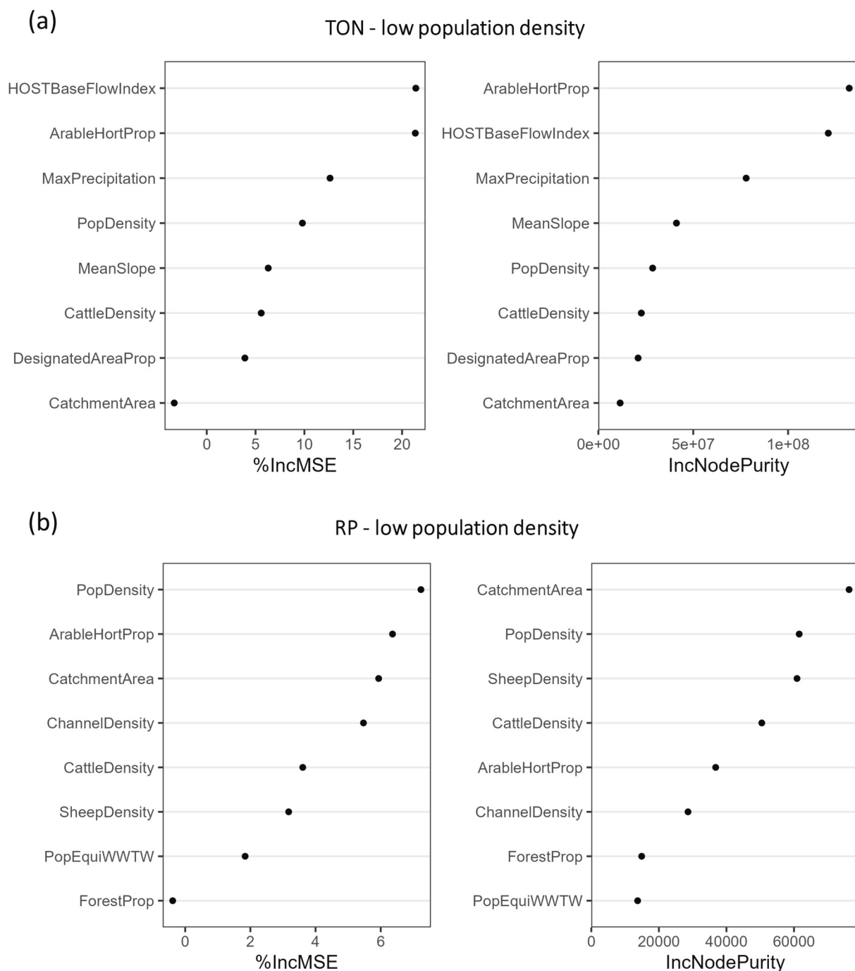
Fig. 5. Variable importance for the random forest for TON in catchments with low population density (a), RP in catchments with low population density (b). In each case the left hand panel shows the permutation importance and the right hand panel the Gini importance.
