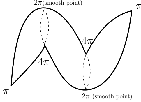
FIGURE 1. The reducible conical metric given by the developing map f(z) = \sqrt{z} \frac{z-3}{z+1} . It can be obtained by gluing three spherical footballs of angle \pi , and has four conical points with angle \pi, \pi, 4\pi, 4\pi .
