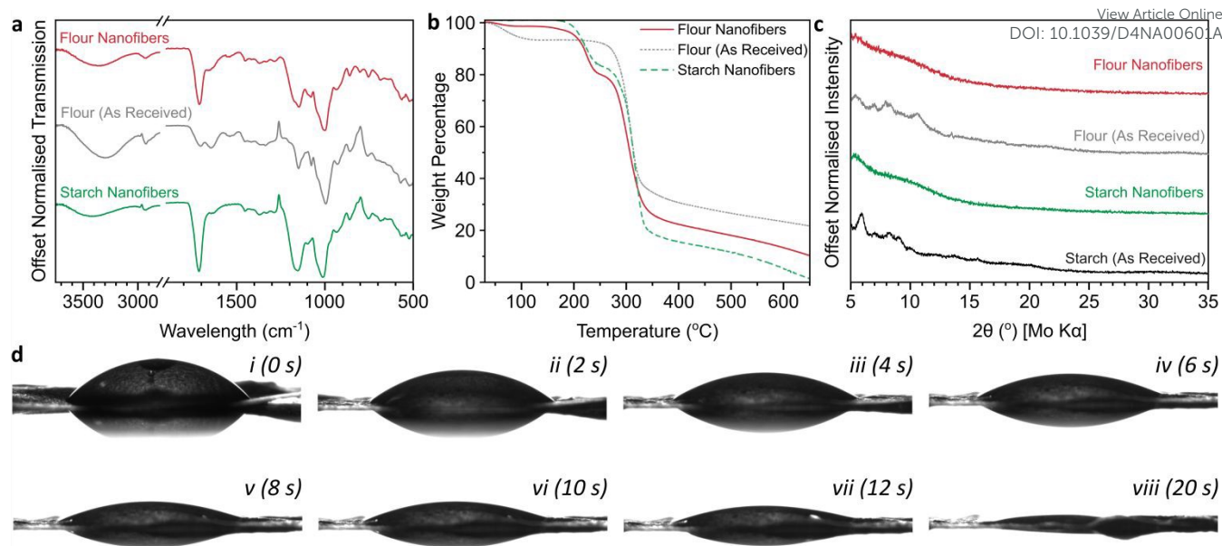
Figure 3. (a) ATR-IR spectra, (b) TGA thermograms under flowing N_2 with 10\text{ }^\circ\text{C min}^{-1} heating, derivatives provided in SI Fig S3, (c) XRD diffractograms using Mo\ K\alpha (0.71 Å), (d) contact angle measurements of nanofiber mat (transferred to a glass slide) as a function of time in 2s increments for the first 12 s (i-vii) and after 20 s (viii).
