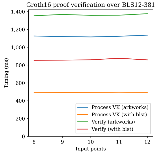
Figure 8: Performance of our implementation of Groth16 zk-proof verification vs. Arkworks' implementation. The performance is independent of the input size, as the plot also shows.
