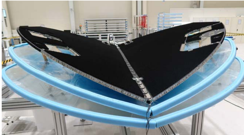
Figure 5-2: V-Groove design (upper), V-Groove STMs with protective covers of lower VGs (lower)
