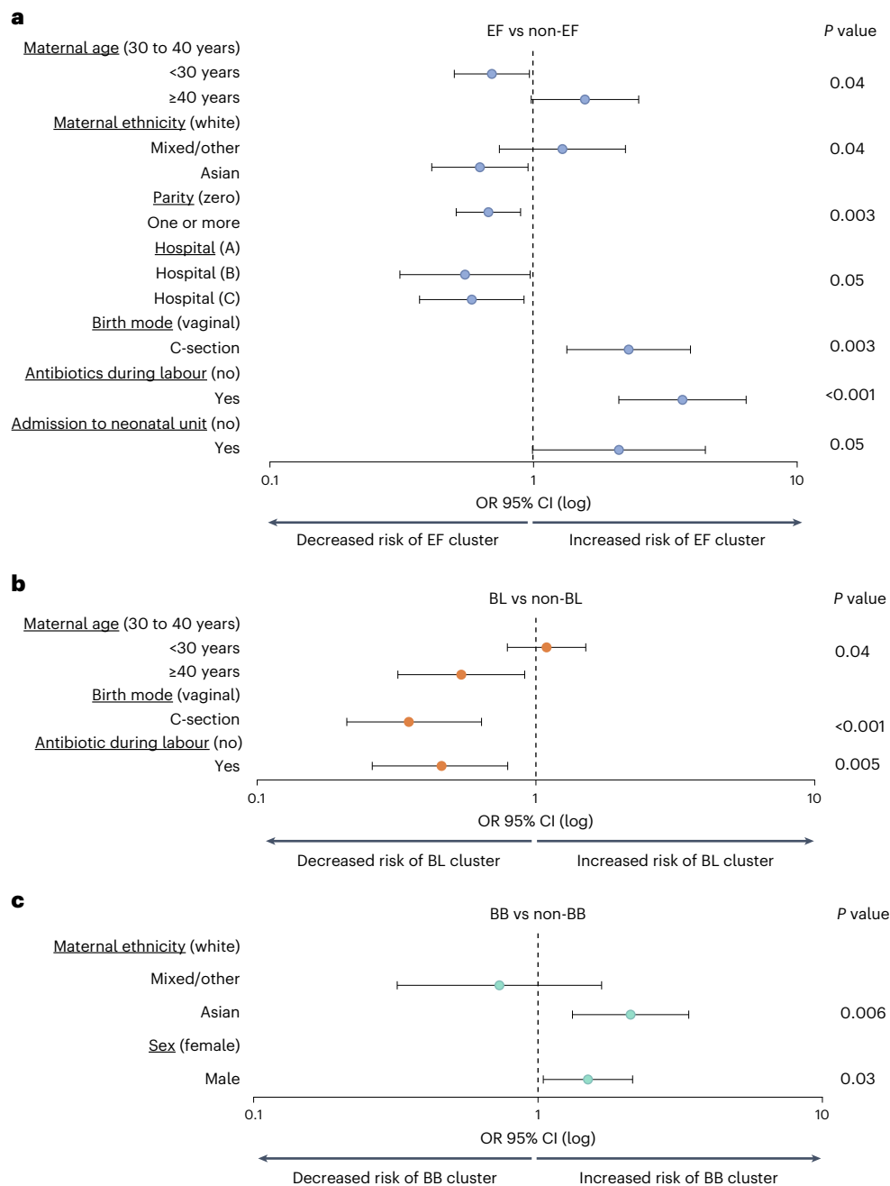
Fig. 2 | Clinical and sociodemographic variables associated with NGM community state in the first week of life ( N = 1,108 ). a–c , Multivariate associations between clinical and sociodemographic variables and each week-1 NGM community state. Three different models were built: EF vs non-EF ( a ), BL vs non-BL ( b ) and BB vs non-BB ( c ). Likelihood ratio tests (two-sided) were used to calculate P values (without FDR correction), with P \leq 0.05 in the multivariate
