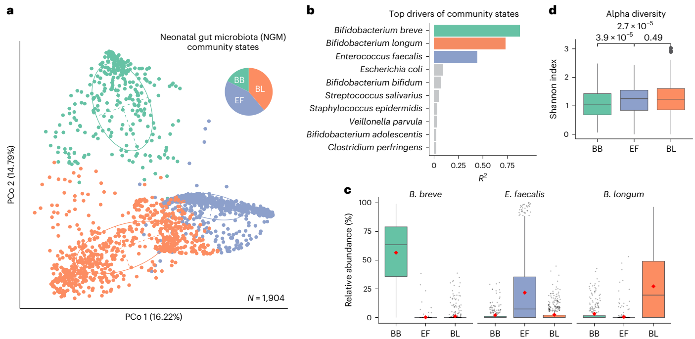
Fig. 1 | Dominant species driving three NGM community states. a , Principal coordinates analysis (PCoA) plots of 1,904 neonatal gut metagenomes sampled within the first 30 days of life and clustered using the PAM algorithm on the basis of species-level JSD. Three distinct NGM community states (optimal number clusters k = 3 ) were identified via PAM clustering. The inset pie chart displays the proportion of the three NGM community states, each labelled according to its primary driver species, namely B. breve (BB, green; N = 336 , 17.6% of the samples), E. faecalis (EF, purple; N = 827 , 43.4% of the samples) and B. longum (BL, orange; N = 741 , 38.9% of the samples). Ellipses encapsulate 67% of the
