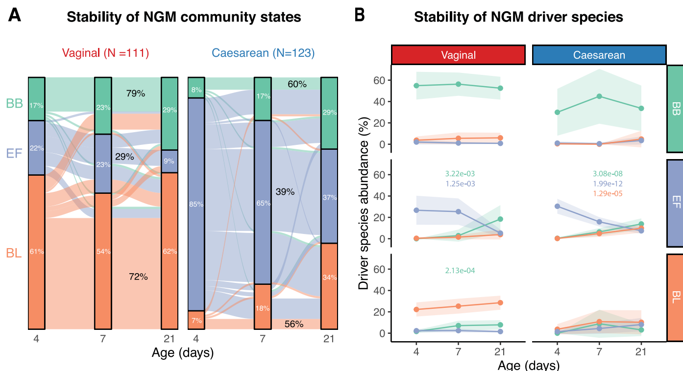
Extended Data Fig. 7 | Colonisation dynamics in neonatal longitudinal samples. (a) Overview of NGM community states of all subjects individually sampled on major neonatal period sampling points day 4, 7 or 21, stratified by birth mode. In VD, N=176/602/156 on day 4, 7, and 21, respectively; In CS, N=184/547/194 on day 4, 7, and 21, respectively. Total samples N=1859. (b) Longitudinal shifts in NGM community states and the levels of driver species from week 1 to week 3, based on subjects longitudinally sampled across days 4, 7, and 21, N=234; VD, N=111; CS, N=123). Community states that remained consistent from first (day 4) to the final neonatal longitudinal sampling (day 7 or/and 21), is depicted as a percentage of their starting pool size (labelled in black). Subjects that began with either BB or BL community state on day 4 were significantly
