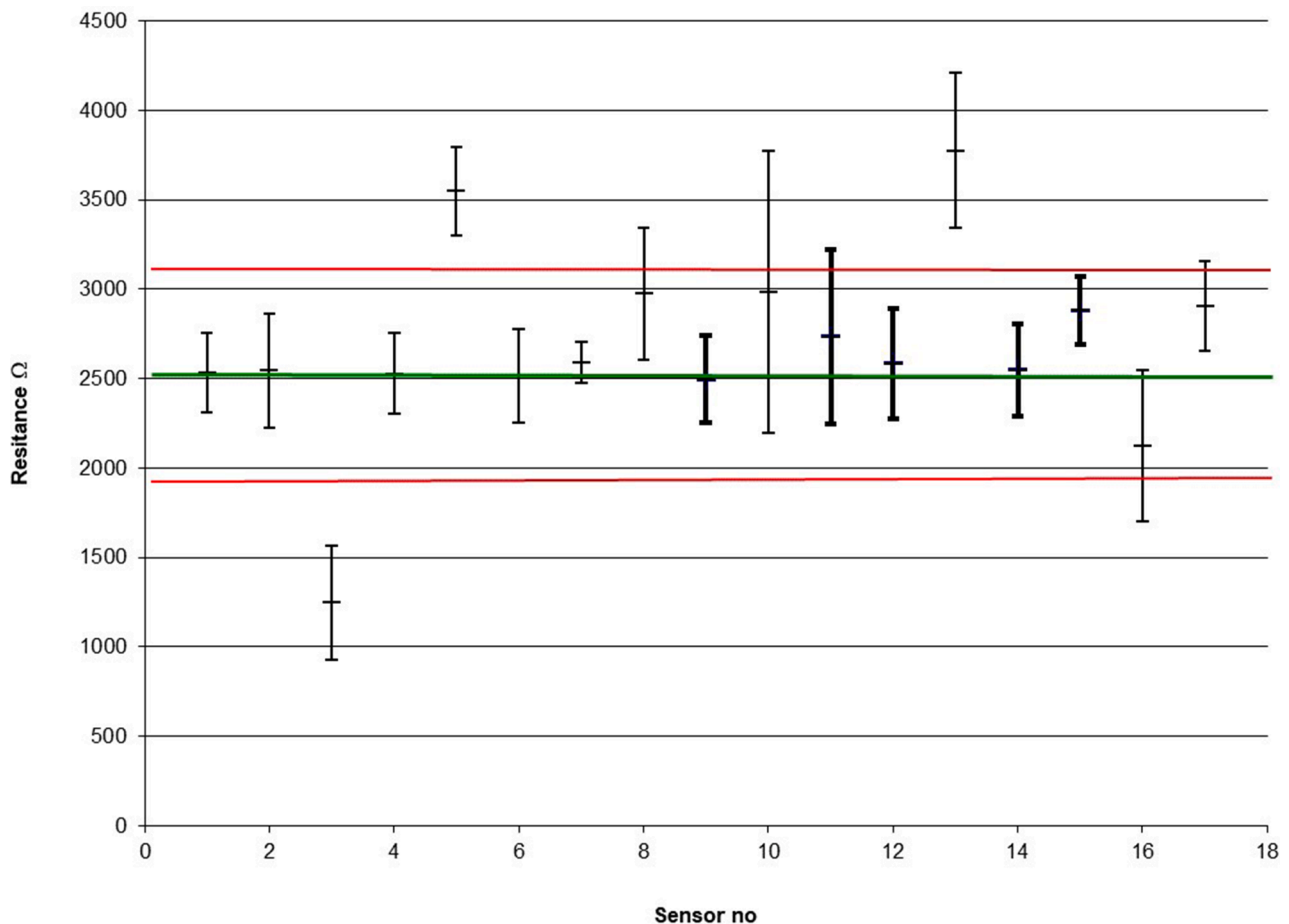
Fig. 6. Performance of a batch of the sensors. Each value is the response of the sensor to a 4.4N load made over six measurements (error bars). Sensors used in the next stage (encapsulation) are in bold . Order left to right the same as in Figure 7. The green line is the population mean and the red lines is the standard deviation from the mean
