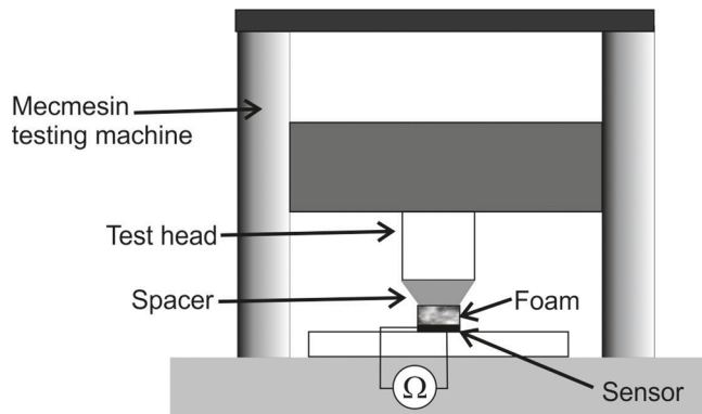
Fig. 2. Experimental set up for testing the force sensors. A Mecmesin testing rig is used to load forces upon a sensor. It uses a foam insert to spread the load across the sensor. The resulting resistance of the sensor is then measured.
