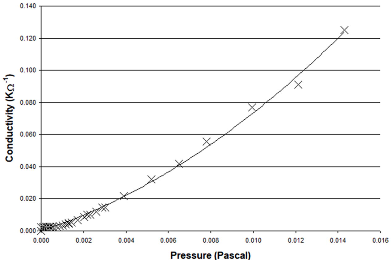
Fig. 4. Characteristic of a single sensor. Increasing pressure is placed on the sensor using a Mecmesin tensile testing machine. The increasing conductivity is the result of increasing contact area between the cloth and the conductive layer. This is supported by the observed quadratic relationship between the conductivity and the pressure imposed.
