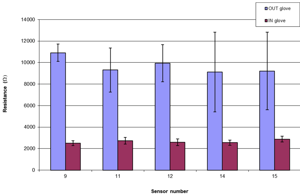
Fig. 7. Resistance response to a 4.4N load of sensors in their normal state outside of a silicone glove (OUT glove) and encapsulated within a silicone glove (IN glove). Overall sensor conductance is lower when inserted into a silicone glove, but variance is also substantially lowered
