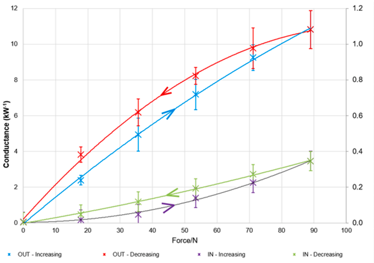
Fig. 5. Characteristic of a single sensor with increasing (blue and mauve) and decreasing (red and green) loads. First outside (OUT) then after embedding in (IN) a silicone composite used to make the prosthetic gloves. Measurements are the conductance, recorded five times after the reading had settled for 10 seconds. Note: The OUT glove readings use a scale ten times the In glove readings.
