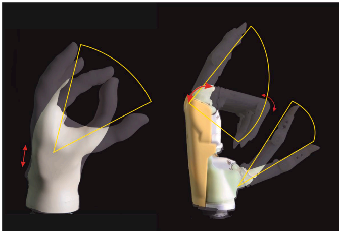
Fig. 1. Range of motion of a typical single degree hand (yellow lines), and that of a multifunction hand (Motion Control and Touch Bionics). The multifunction hand has independent motion of thumb and finger, while the digits in the single axis hand are linked. The range of motion of the single degree of freedom is less than 50°. The resulting motion causes the glove to become stretched as the hands close, the key points of stretch are indicated in red.
