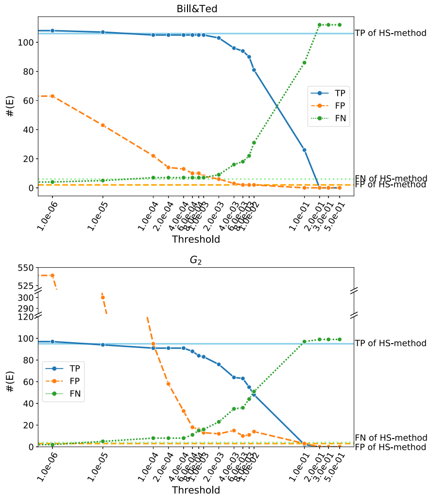
Fig. A.25. The number of true-positive (TP), false-positive (FP), and false-negative (FN) edges found in the causal structure of the RCP -method using different thresholds. The horizontal lines show TP, FP, and FN of the causal structure of the HS -method.
