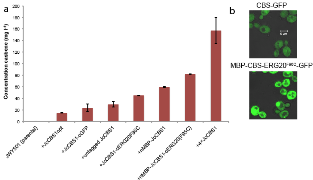
Figure 2 | Engineering casbene production in yeast. (a) Different protein solubility tags on J. curcas casbene synthase (JcCbs1p) improved casbene titer, with the preceding letter representing the fusion of the tag on the N- or C- terminus of Cbsp. All JcCBS1 variants were integrated into the GGPP-producing parent strain, JWY501. Strain JWY509, containing four copies of JcCBS1 , was used as the parent for all P450 testing in subsequent studies. Data represent the averages of three replicate cultures; error bars show s.d. (b) GFP-tagging experiments with JcCbs1p reveal increased expression and protein stability with solubility tags. Confocal microscopy studies show low expression from a single integrated copy of GFP fused JcCbs1p in yeast (top). A single integrated copy of three tag JcCBS1 (producing nMBP-JcCbs1-cErg20[F96C]-cGFPp) results in increased expression levels (bottom).
