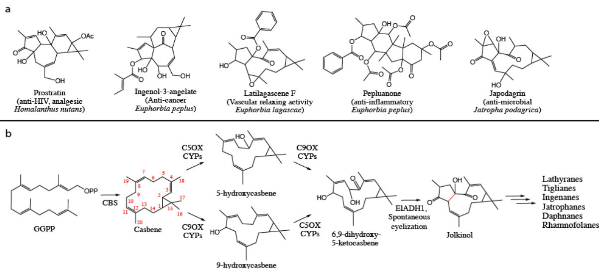
Figure 1 | Euphorbiaceae diterpenoid biosynthetic pathways originate from casbene. (a) Structures of bioactive Euphorbiaceae diterpenes. (b) Proposed pathway for the production of medicinal Euphorbiaceae diterpenoids begins with geranylgeranyl diphosphate (GGPP) from the DXP pathway in plants, which is cyclized by casbene synthase (CBS) and subsequently oxidized by numerous P450s. Enzymes required to form jolkinol C in both J. curcas and E. lathyris have been functionally characterized. C9OX CYP (EiCYP71D445p/JcCYP71D495p) homologs oxidize the C-9 position of casbene, while C5OX CYP (EiCYP726A27p/JcCYP726A35p/JcCYP726A20p) homologs oxidize the C-5 position of casbene. Consequently, both enzymes have been shown to catalyze the hydroxylation of C-6 position of casbene, the formation of a carbonyl at which position has been postulated to result in the tautomerization and spontaneous ring closure forming jolkinol C. Hamberger and colleagues have shown the necessity of the alcohol dehydrogenase ELADH1p to form jolkinol C in vitro using E. lathyris enzymes. Additional steps towards production of decorated diterpenes are diverse and unknown.
