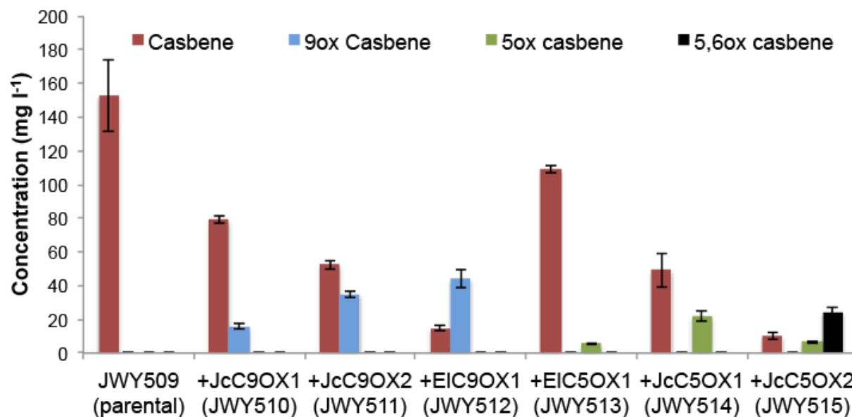
FIGURE 3 | Titers of casbene, singly- and doubly- oxidized casbanes (sum of hydroxy and oxo forms), detected in the presence of different C9OX and C5OX CYP variants. All CYP variant constructs were individually cointegrated with the J. curcas CPR ( JcCPR1 ) into the 911b locus of the high titer casbene strain JWY509. The formation of 9-ketocasbene has been shown to be a dead-end product and is likely due to overactivity of C9OX on an accumulating 9-hydroxycasbene, resulting in double oxidation at the C-9 position. Thus, we determined the overall activity of the CYPs by the total production of these products, as we presume that the 9-hydroxycasbene product of these enzymes will be consumed in the presence of a C5OX CYP, which has been shown to act on both casbene and 9-hydroxycasbene, but not 9-ketocasbene in vitro (Luo et al. 2016). Cultures were extracted after 48 hours and analyzed for oxidized casbane production by GC-MS. EIC9OX1 outperforms all C9OX CYPs in C-9-oxidized casbene production, while JcC5OX2 outperforms all the other C5OX CYPs in production of C-5/C-6 oxidized casbene. Data represent the averages of three replicate cultures; error bars show s.d.
