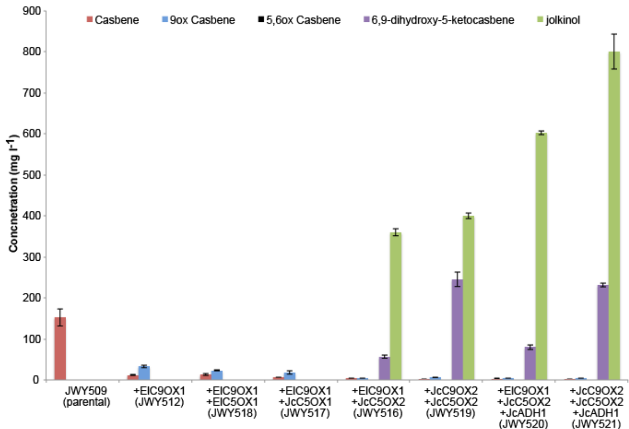
Figure 4 | Production of 6,9-hydroxy-5-ketocasbene and jolkinol C with different C9OX CYP/C5OX CYP combinations and short chain ADH variants. C5OX CYPs were screened for jolkinol C production when expressed with the most productive C9OX CYP, EIC9OX1p. Only JcC5OX2p formed any detectable level of jolkinol C. Additionally, we integrated this CYP into the best J. curcas C9OX CYP parental strain containing JcC9OX2p. It is important to note that EIC5OX1p produced low titers of C-5 oxidized casbanes in JWY509 and produced low levels of 9-keto-5-hydroxycasbene, a purported dead end product, while producing no triply oxidized casbanes nor jolkinol C. All strains were cultured in 2ml of YPG media in milliliter plates, grown for 48 h, and the culture medium analyzed for casbene (red bars) and C-9 oxidized casbene (blue bars) by GC-MS, while all other compounds were measured by HPLC-UV. Bars represent mean values \pm 1 s.d. of three replicate cultures. All compounds were quantified using authentic standards purified from high-producing strains.
