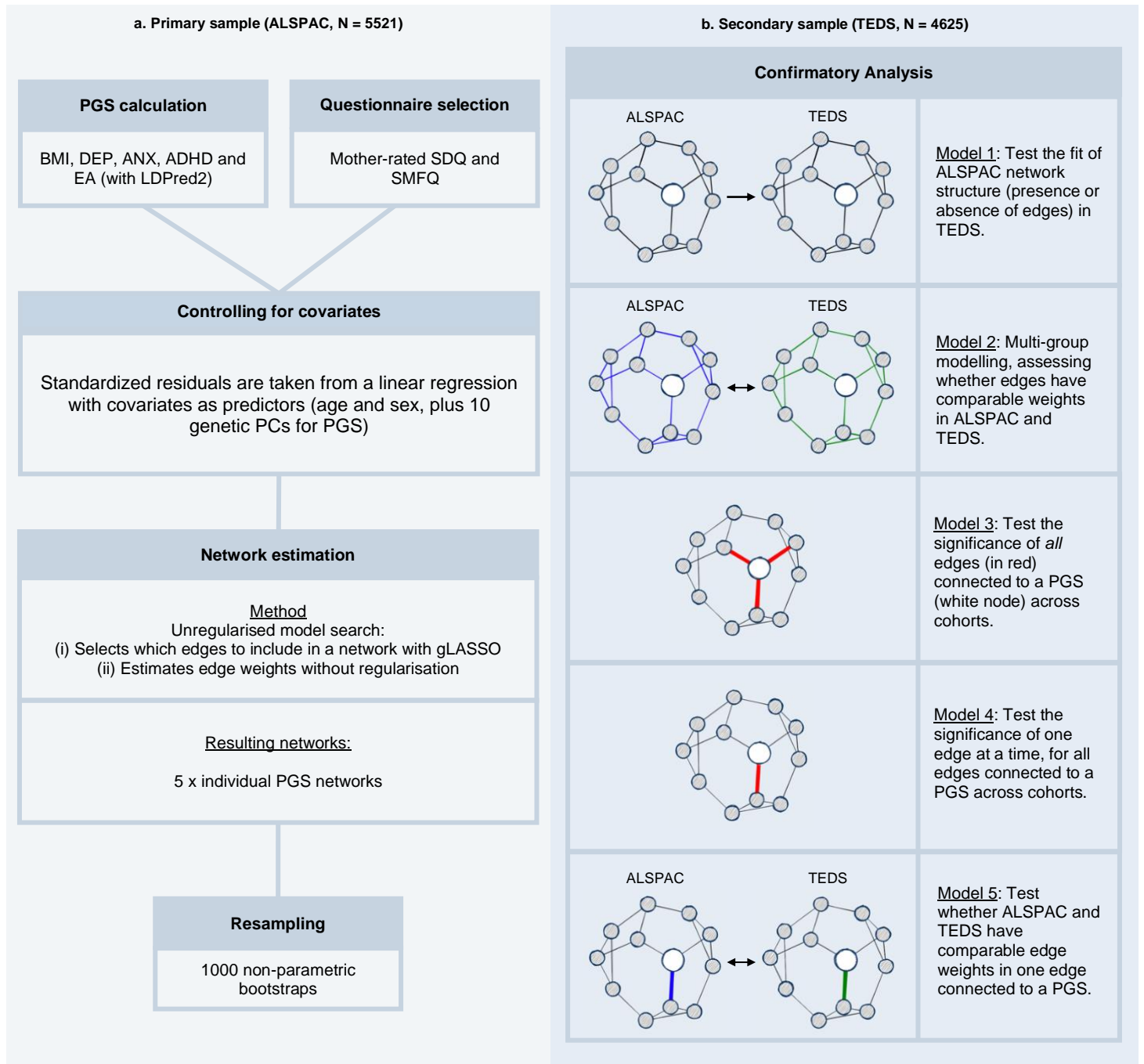
Figure 1: Analysis flow of the study, including network analysis in ALSPAC (a) and replication in TEDS (b)
