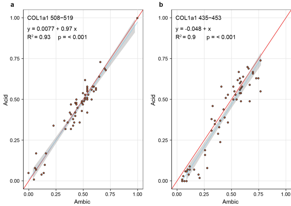
Extended Data Fig. 7 | Comparison of deamidation between proteomic extraction methods. a,b , Scatter plots of COL1 \alpha 1508-519 (P1105; a ) and COL1 \alpha 1435-453 (P1706; b ) deamidation values for AmBic-based and acid-based extractions. The blue line and grey area indicate the mean of the loess
