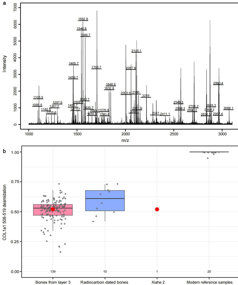
Extended Data Fig. 6 | The Homo sp. rib specimen (Xiahe 2) identified by ZooMS. a. MALDI-TOF MS spectrum of Xiahe 2. b. Comparison of deamidation values of Xiahe 2 with values of faunal specimens from layer 3 (n = 139, including Xiahe 2, indicated by the red point), the radiocarbon-dated bone specimens (-50–30 ka, n = 10, Supplementary Data 2) and modern reference samples (n = 20). Here, the value of 1 indicates no deamidation while the value of 0
