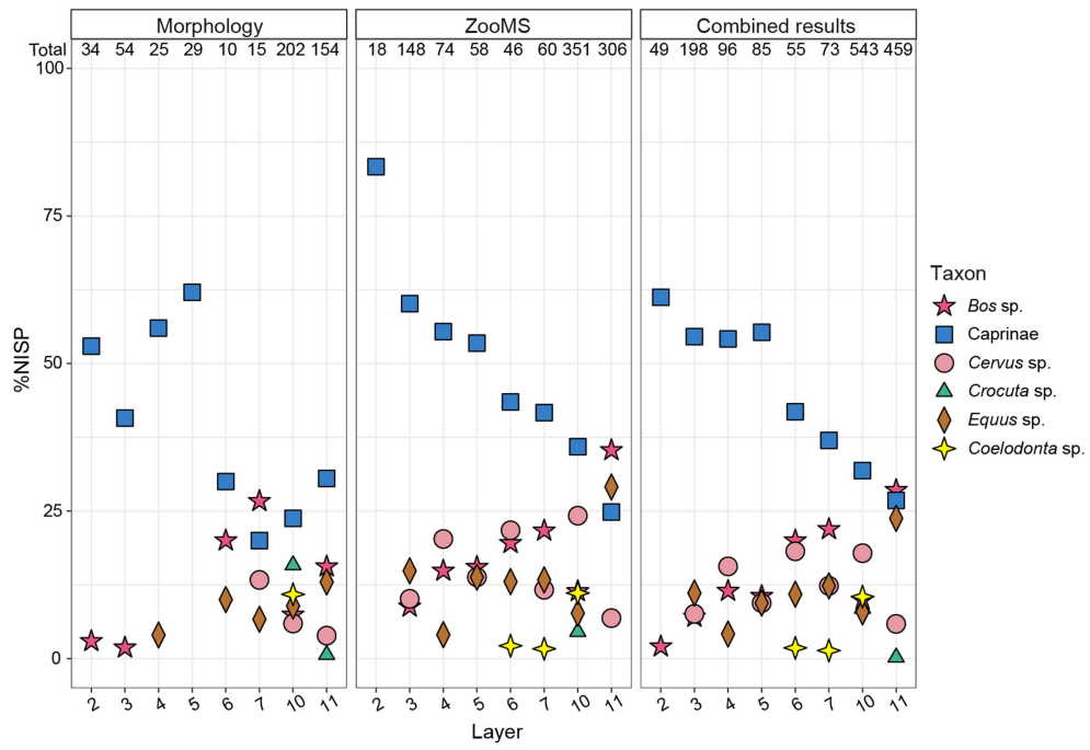
Extended Data Fig. 3 | Relative species composition of BKC, for selected taxa. Proportions of selected taxa identified using morphology, ZooMS, and both combined, per layer. The total NISP for each layer is given at the top. The combined data is based on Extended Data Table 1 ( n = 1,558 ).
