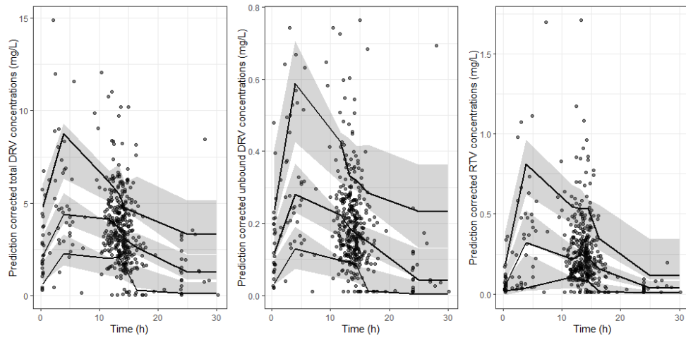
Figure 4. pcVPC plots for total DRV (left), unbound DRV (middle) and RTV (right) concentrations. Black points represent observed concentrations. Solid black lines represent the 10 th , 50 th and 90 th percentiles of observed concentrations. Grey areas represent the 95% confidence interval of the 10 th , 50 th and 90 th percentiles of simulated concentrations.
