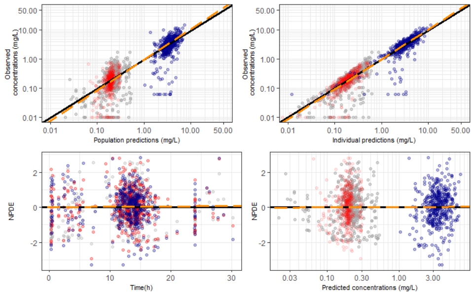
Figure 3. Goodness of fit plots from the final joint model. Red, blue and grey points are unbound DRV, total DRV and RTV concentrations, respectively. NPDE is the normalized prediction distribution error. Solid lines represent identity lines (top plots) or theoretical mean of NPDE (bottom plots). Orange dashed lines are the regression lines.
